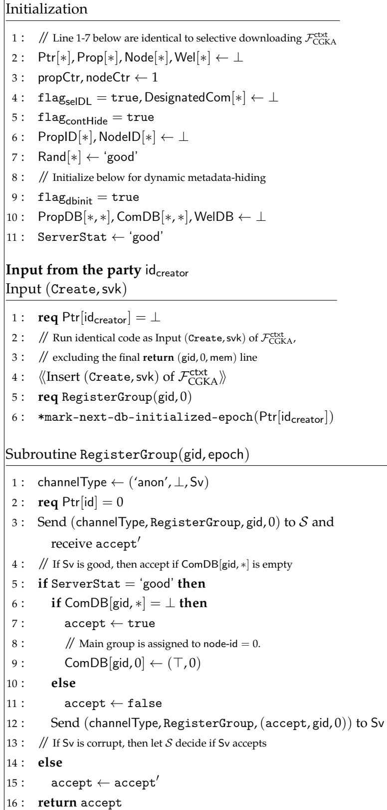
FIGURE 5.43: The ideal MH-CGKA functionality \mathcal{F}_{\text{CGKA}}^{\text{mh}} : Create function for honest parties. For better readability, we outsource the lines identical to \mathcal{F}_{\text{CGKA}}^{\text{txt}} to Figure 5.5. Note that the Create function is invoked only once by the previously designated party \text{id}_{\text{creator}} . (Only one \text{id}_{\text{creator}} exists.)
