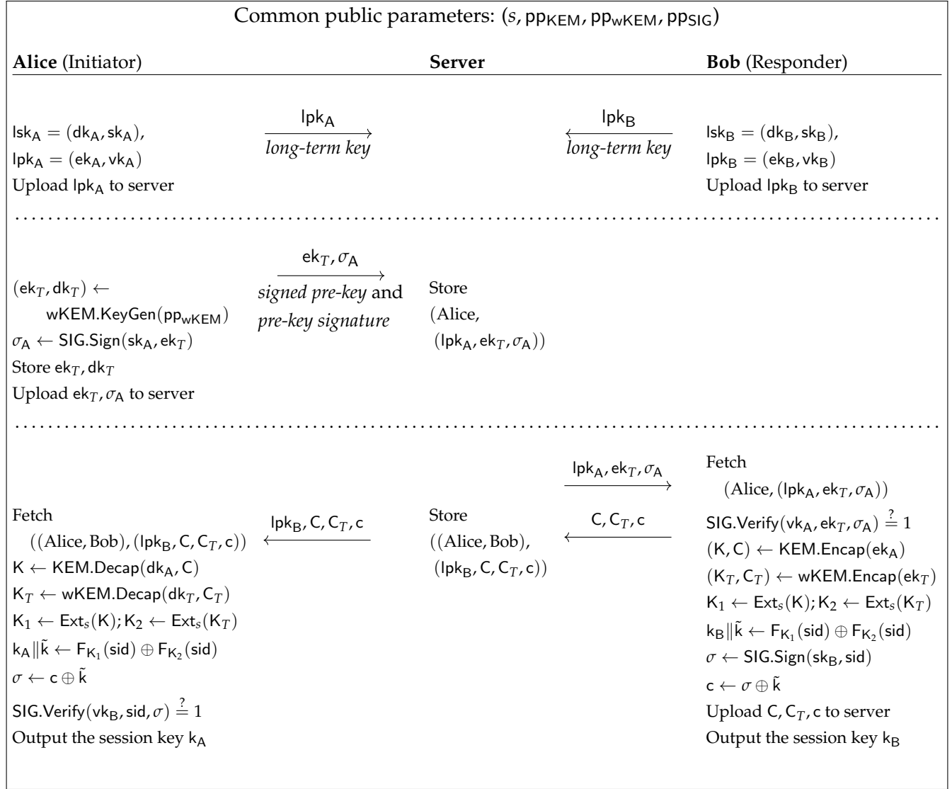
FIGURE 3.4: Post-quantum Signal handshake protocol based on our Signal-conforming AKE protocol \Pi_{SC-AKE} that reuses the same first message (i.e., signed pre-key and pre-key signature). The session identifier is defined as sid := A || B || lpk_A || lpk_B || ek_T || C || C_T . Alice and Bob only need to upload their long-term (public) keys to the server once, and the signed pre-key and pre-key signature are reused by multiple responders throughout some interval.
