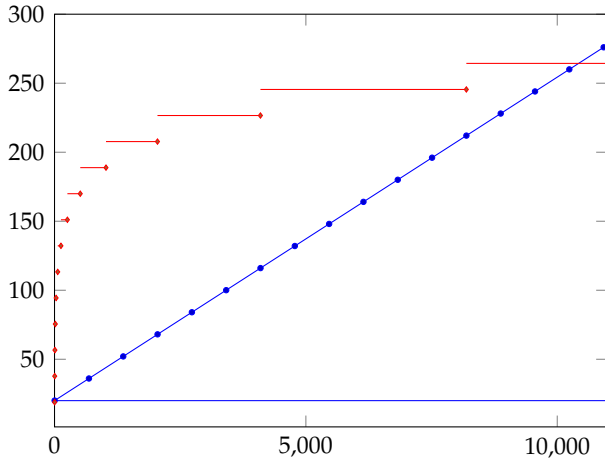
(A) Bilbo640 vs. Frodo640
