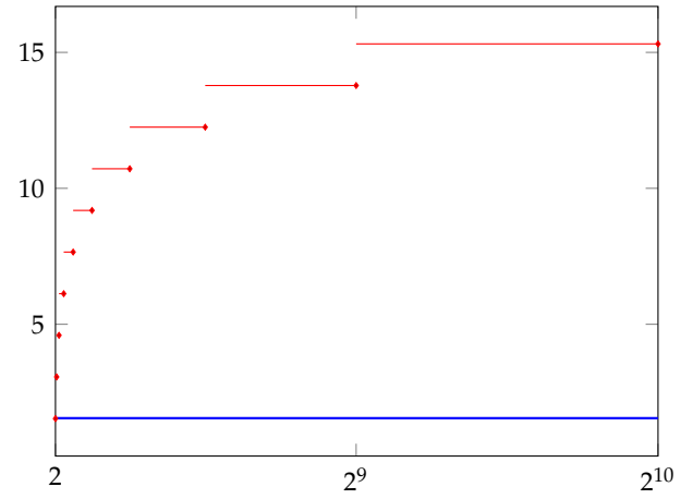
(B) Ilum512 vs. Kyber512
