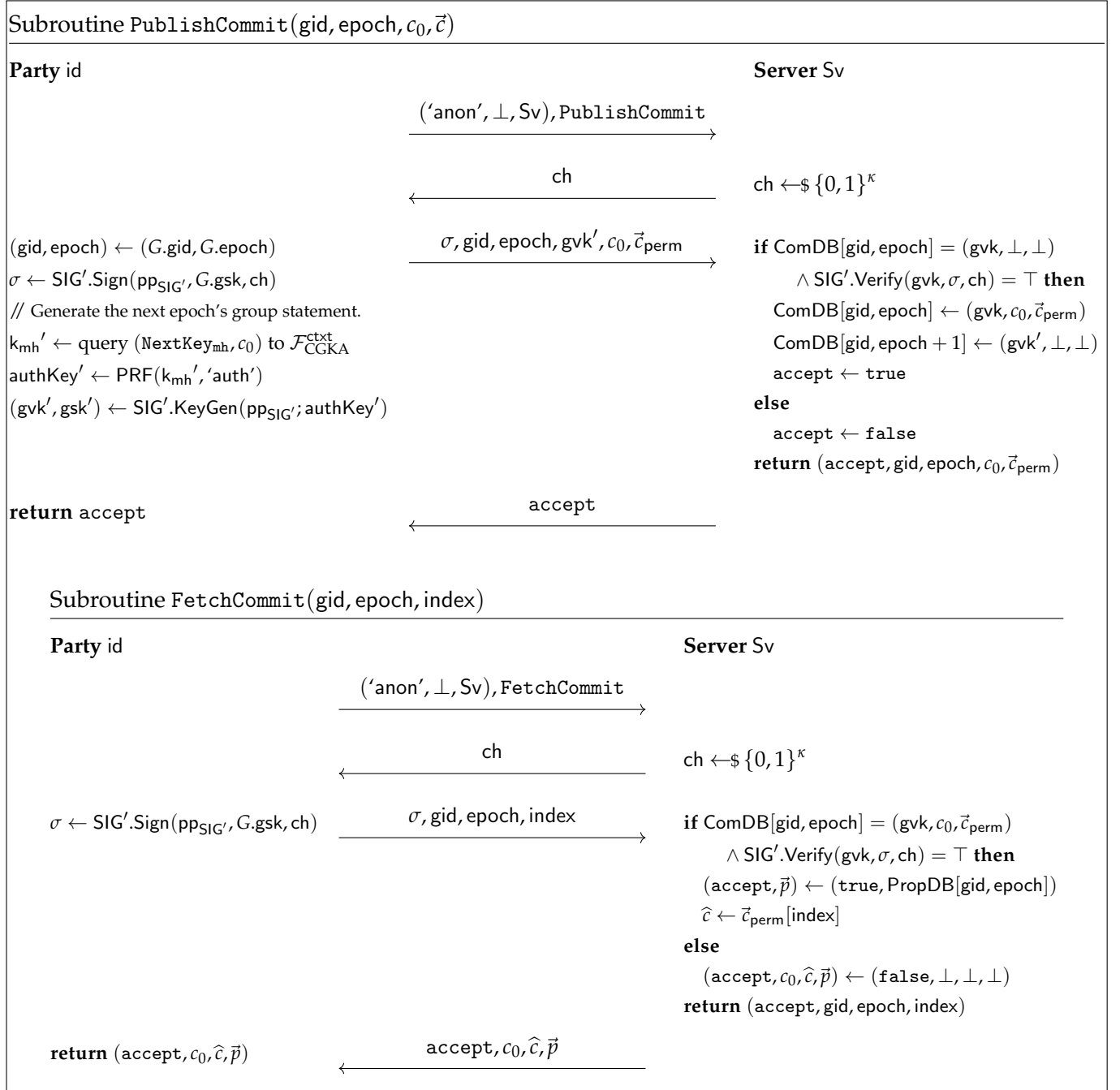
FIGURE 5.39: Subroutines for metadata-hiding CGKA protocol W^{\text{mh}} in the \mathcal{F}_{\text{CGKA}}^{\text{ctxt}} -hybrid model: Publish and fetch commit messages. Party id and the server Sv are connected via a client-anonymized authenticated channel.
