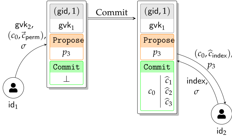
FIGURE 5.35: Left: a commit sent by id_1 . Right: a subsequent process made by id_2 . Member-dependent commits \vec{c}_{perm} := (\hat{c}_1, \hat{c}_2, \hat{c}_3) are randomly permuted and id_2 specifies an index to fetch the commit from the server. Challenges sent by the server are omitted for readability.
