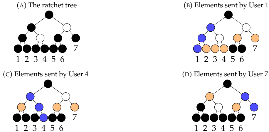
FIGURE 5.57: Example of the TreeKEM ratchet tree with blank nodes. The numbers indicate party identities. Figures 5.57b to 5.57d: sending encryption keys (blue) and ciphertexts (orange) when party 1, 4 or 7 commits, respectively.
