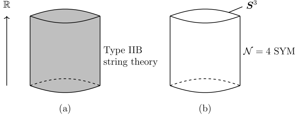
Figure 4.1: (a) The Type IIB string theory in \mathbb{R} \times B^4 . (b) The \mathcal{N} = 4 SYM in \mathbb{R} \times S^3 .
