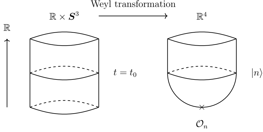
Figure 3.1: A state/operator correspondence. The infinite past t = -\infty on \mathbb{R} \times \mathbf{S}^3 is moved onto the origin on \mathbb{R}^4 by the Weyl transformation. A state |n\rangle at t = t_0 corresponds to a local operator inserted at the origin.
