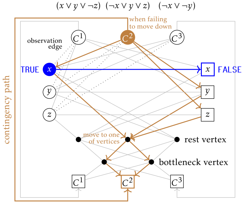
Figure 10.8: MAPPCF instance and solution reduced from SAT. The corresponding formula is (x \vee y \vee \neg z) \wedge (\neg x \vee y \vee z) \wedge (\neg x \vee \neg y) . Dotted lines are edges that are not used in the plans.
