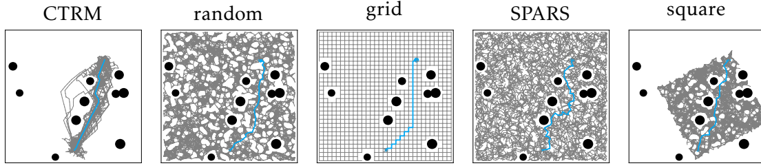
Figure 11.4: Constructed roadmaps for one agent in the Basic scenario. The blue line is a path in a solution. Parameters are: CTRM: n_{\text{traj}} = 25 ; random: 3,000 samples; grid: 32 \times 32 ; square: the middle density.
