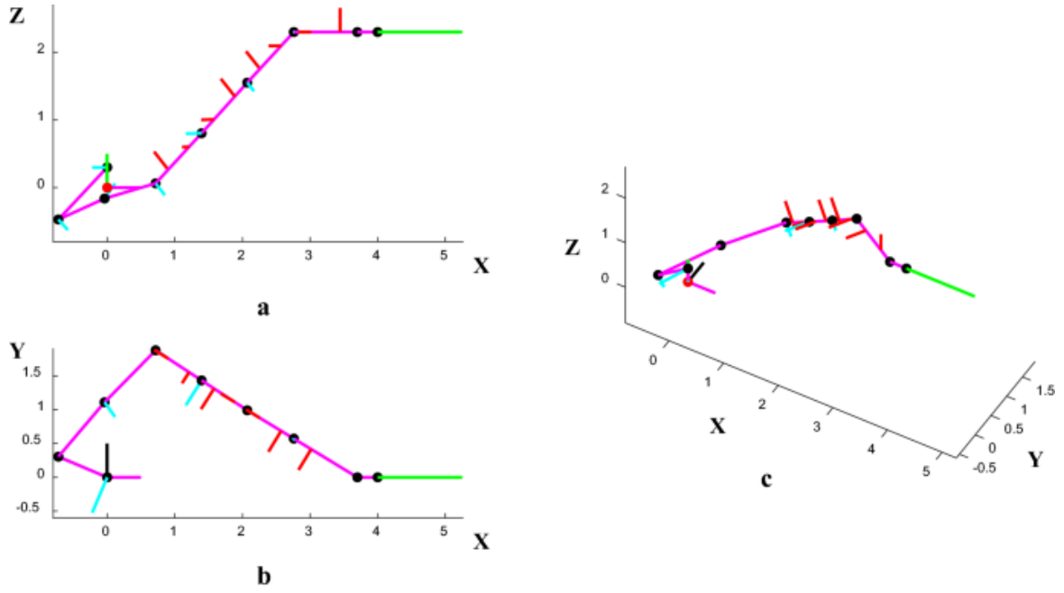
Fig. 4.2. The simulation arm and flying watch thrusts under WACAIE-I when the end effector reaction force is [125,0,0] N (RLR = 24.1%). a Front view. b Top view. c 3-D view
