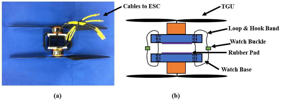
Fig. 2.11. Propeller flying watch prototype (propeller TGU + modified bar belt). a. Photo. b. design. This figure is adapted from [16].
