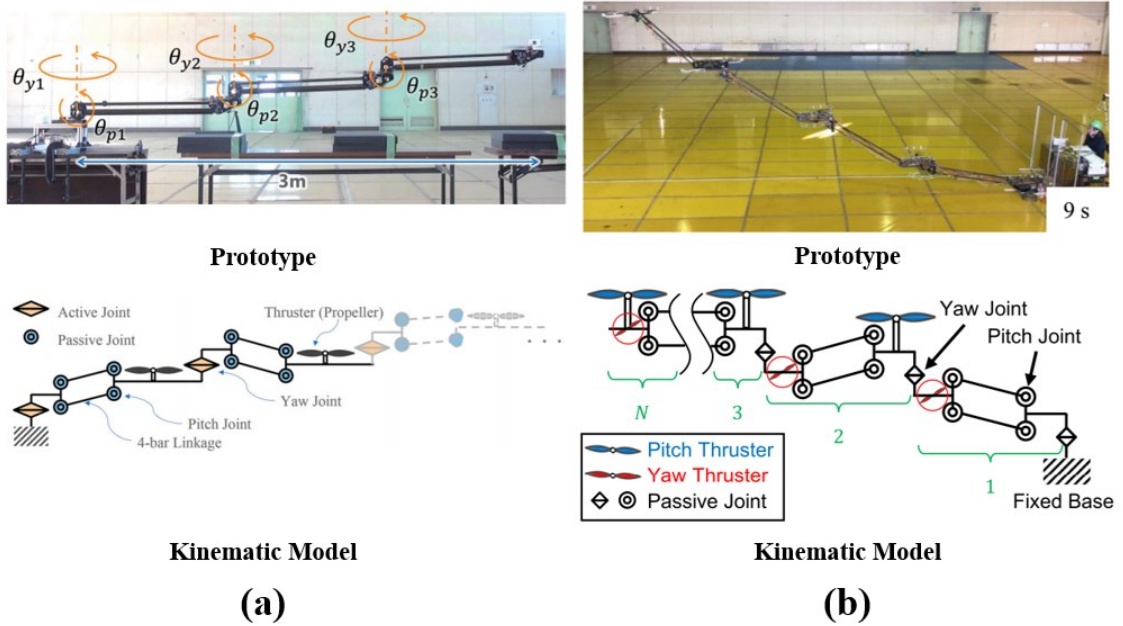
Fig. 1.5. Air thrust driven robotic arms. (a) Hiryu-I. (b) Hiryu-II. (a) is adapted from [13] © 2018 IEEE. (b) is adapted from [15] © 2020 IEEE
