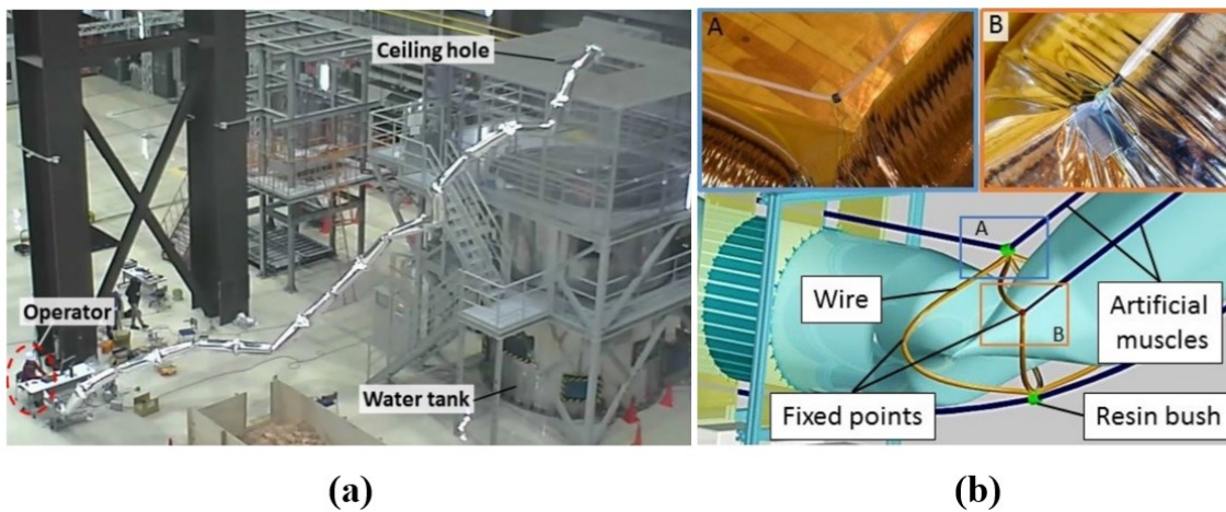
Fig. 1.1. An example of passive force counteraction long robotic arm. The arm is proposed in [3], called Giacometti Arm. (a) Demonstration of Giacometti Arm. (b) Detailed arm design of Giacometti Arm. This figure is adapted from [3] © 2017 IEEE.
