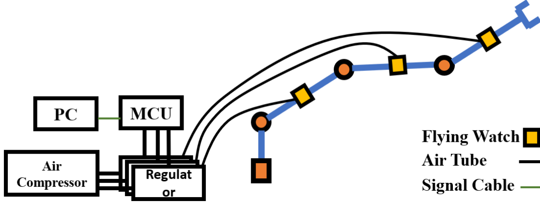
Fig. 2.4. The hardware system of propellerless flying watches. This figure is adapted from [33].
