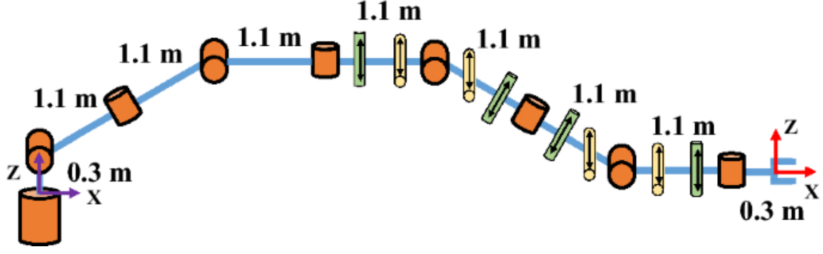
Fig. 4.1. The setup of the simulation robotic arm and flying watches.
