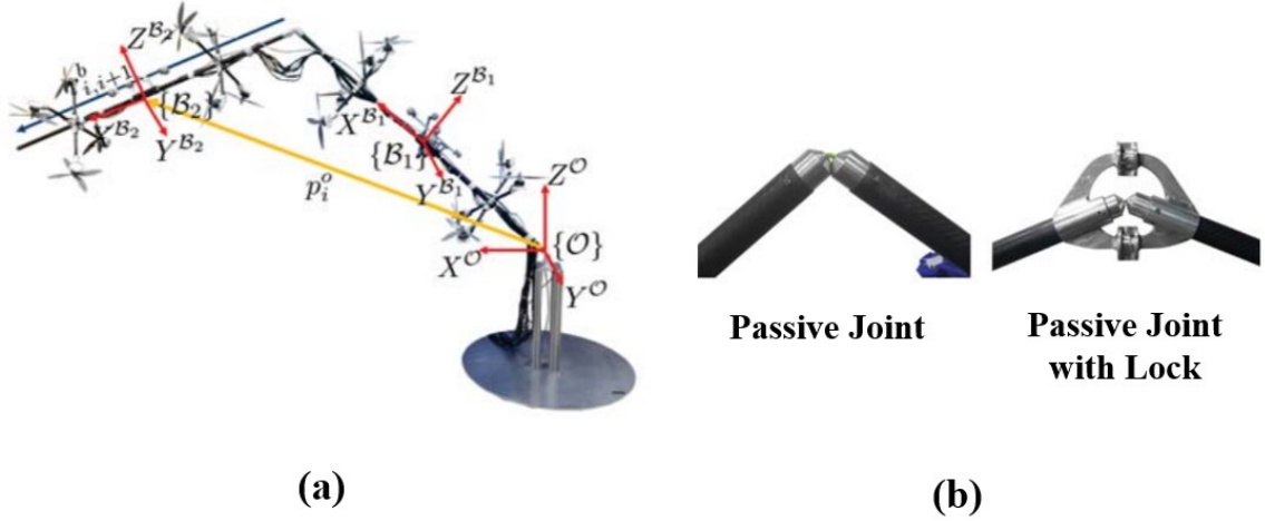
Fig. 1.2. An example of active force counteraction long robotic arm. The arm is proposed in [14], called LASDRA. (a) Overall view of LASDRA. (b) Passive joint design of LASDRA. This figure is adapted from [14] © 2018 IEEE.
