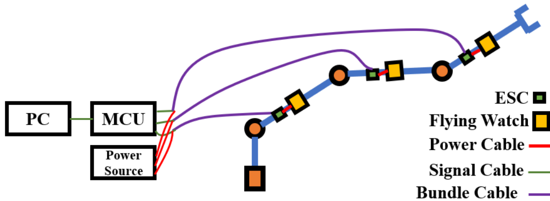
Fig. 2.3. The hardware system of propeller flying watches.
