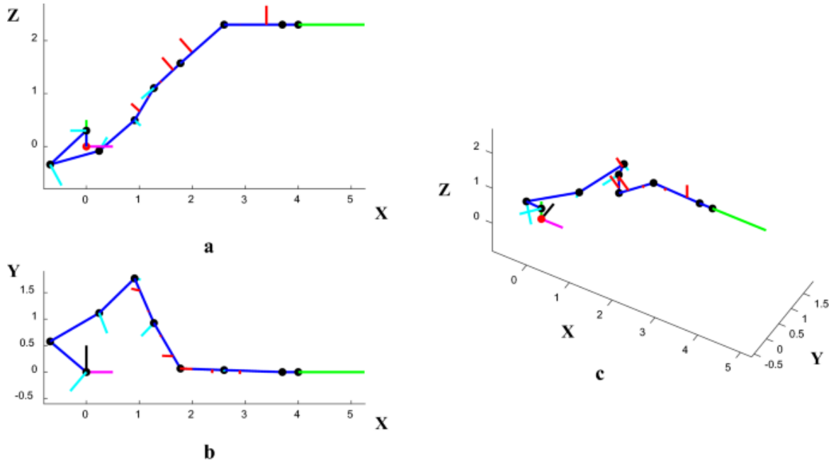
Fig. 4.3. The simulation arm and flying watch thrusts under WACAIE-II when the end effector reaction force is [125,0,0] N (RLR = 35.6%). a Front view. b Top view. c 3-D view
