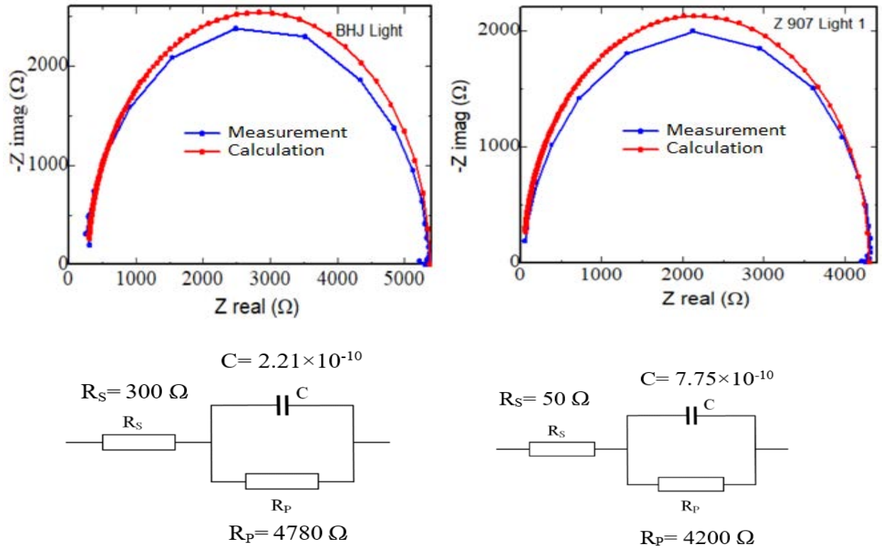
Figure 5.10. The consistency of Z image and Z real for BHJ and Z907 calculations towards the measurements
