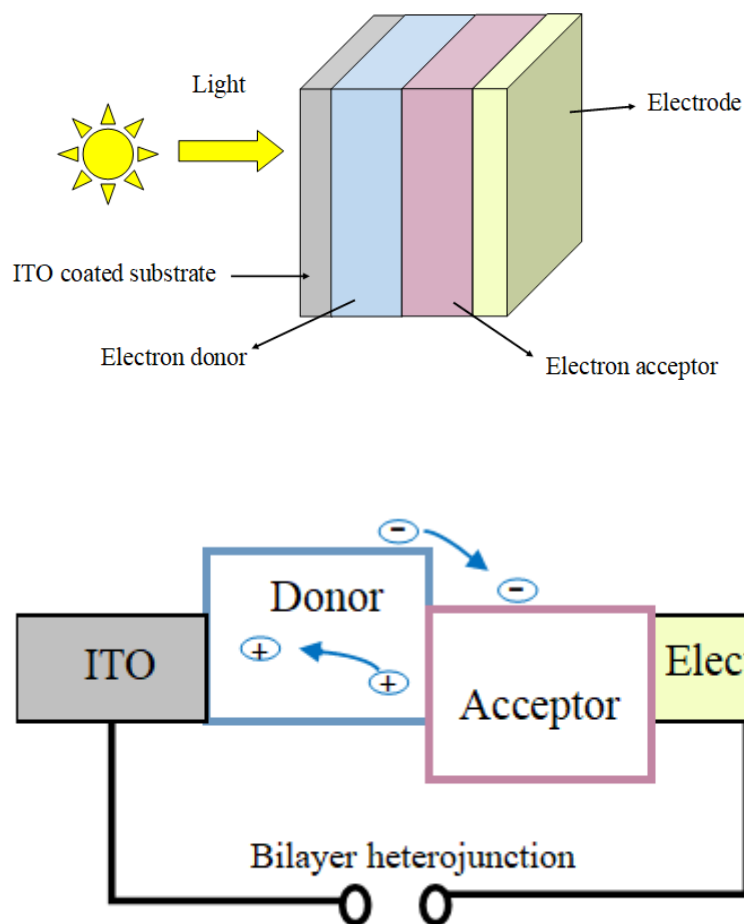
Figure 1.3: a) Device structure of an organic bilayer heterojunction solar cell b) the energy flow diagram of a bilayer heterojunction cell
