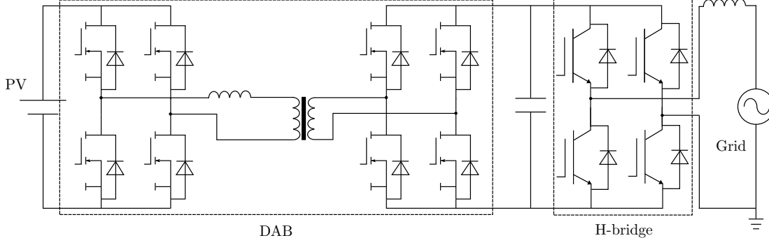
Figure 2.4: DAB application in PV systems.
