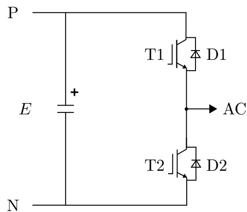
Figure 1.4: Conventional two-level PV inverters.
