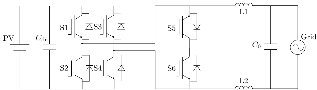
Figure 2.2: HERIC topology.
