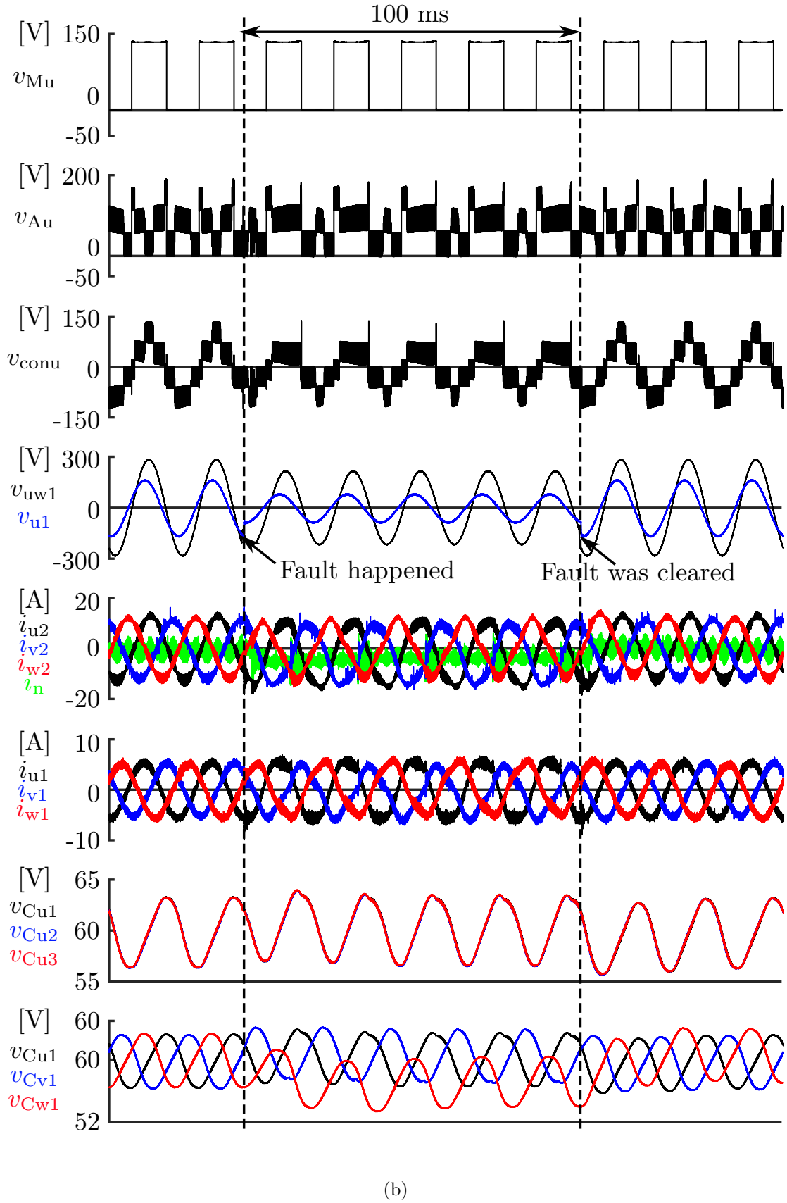
Figure 6.8: Experimental waveforms during SLG fault where E = 135 V and v_{u1} dropped by 50 %: a) two-cell inverter circuit, b) three-cell inverter circuit.
