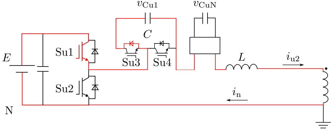
Figure 4.6: Example of current path when v_{Cu1} is charged.
