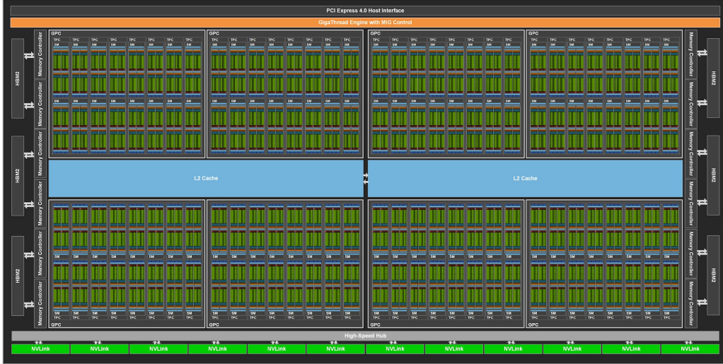
Figure 2.6: NVIDIA A100 GPU architecture
