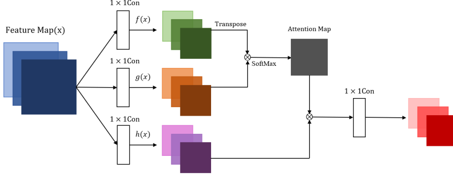
Figure 4.3: Self Attention Architecture
