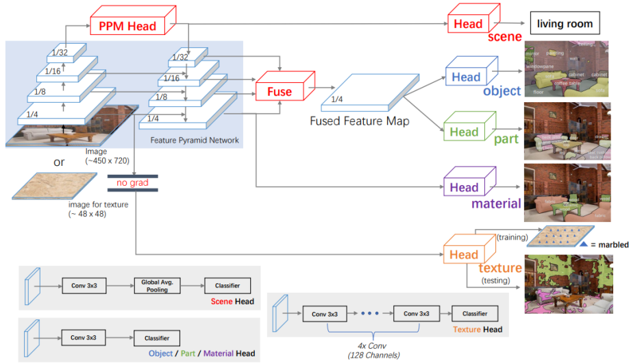
Figure 4.8: UPerNet[129]
