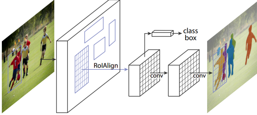
Figure 4.7: Mask R-CNN[46]
