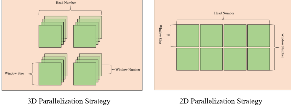
Figure 4.16: Parallelization Strategy
