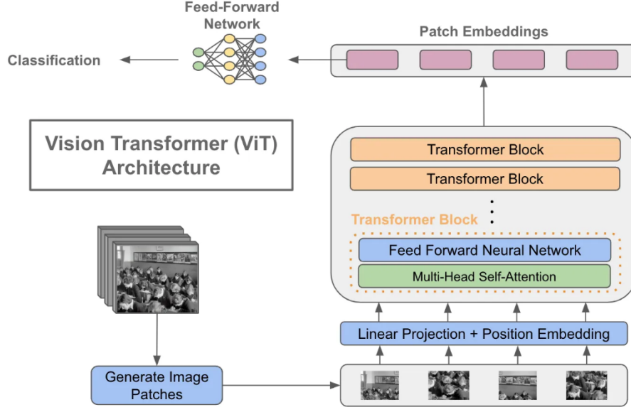
Figure 4.5: Vision Transformer[15]
