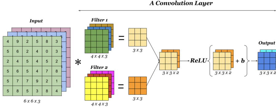
Figure 2.2: A CNN architecture
