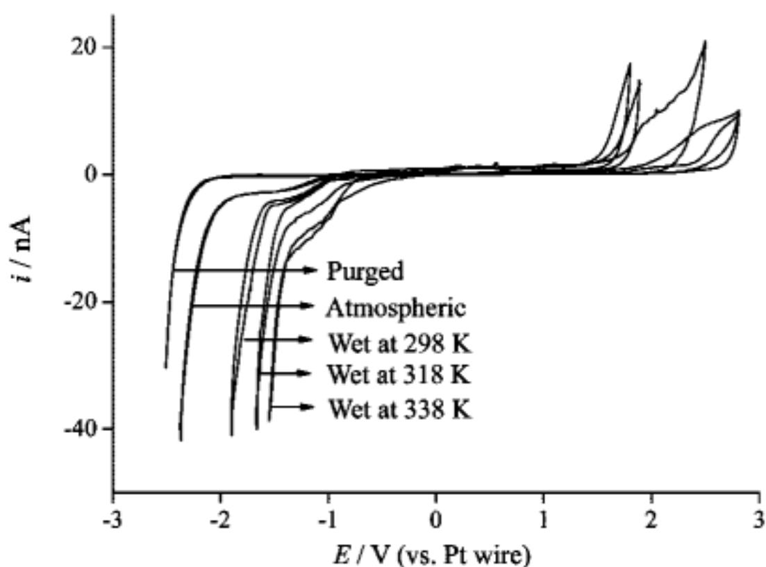
Figure 2.5: ECW from [EMIM][NTf 2 ] at several conditions, i.e., vacuum-dried (purged), atmospheric, and wet conditions. CV was carried out on 10 \mu m Pt electrode vs Pt wire (0.3 mm). Scan rate was 100 mV/s. Reprinted with permission from [76]. Copyright (2008) American Chemical Society
