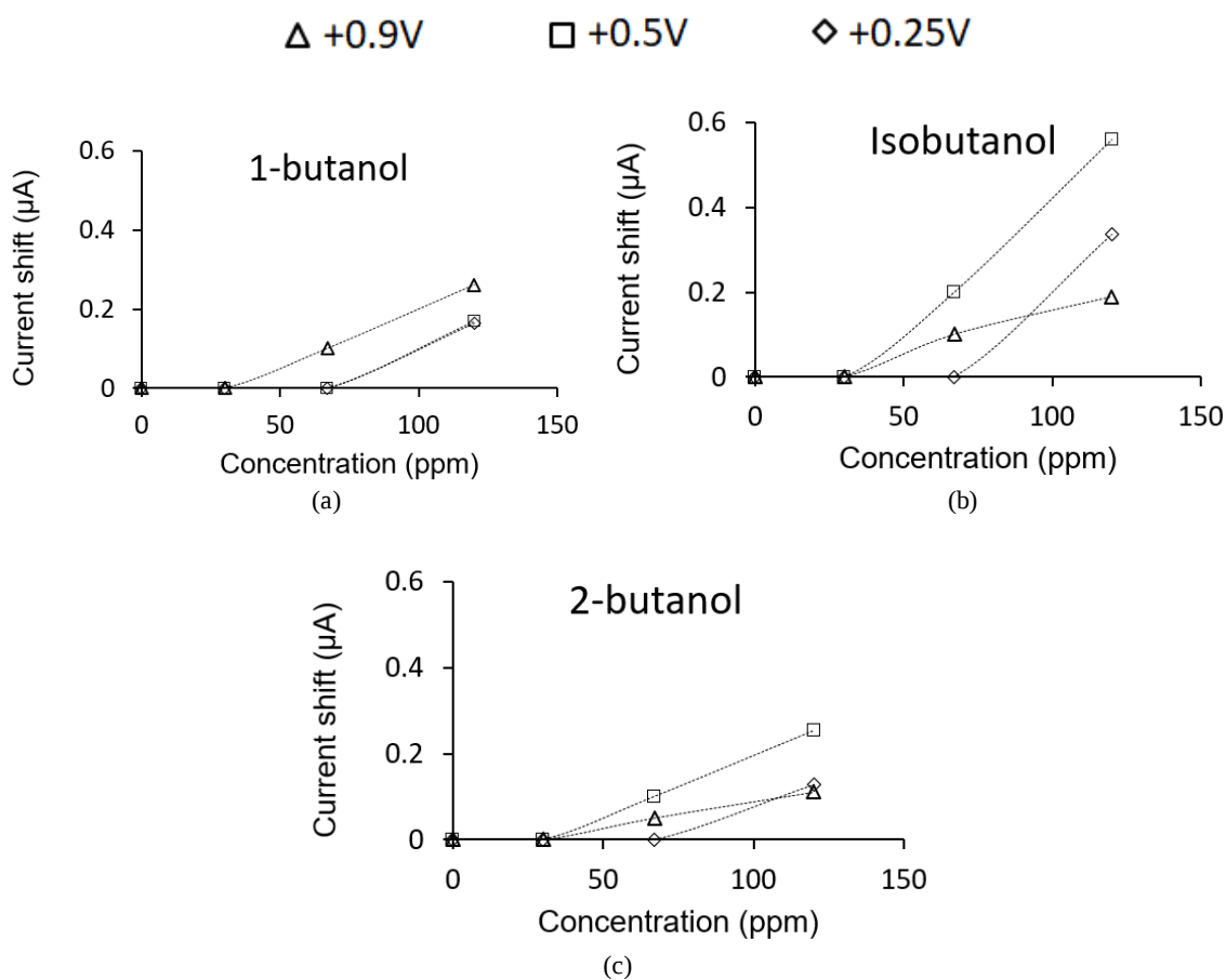
Figure 4.8: Mean sensor response for IDAs with [EMIM][Ac] at three positive E_s (+0.25 V, +0.5 V, and +0.9 V) vs. Ag/AgCl against different concentrations of; (a) 1-butanol; (b) isobutanol; (c) 2-butanol. Reprinted from [98]
