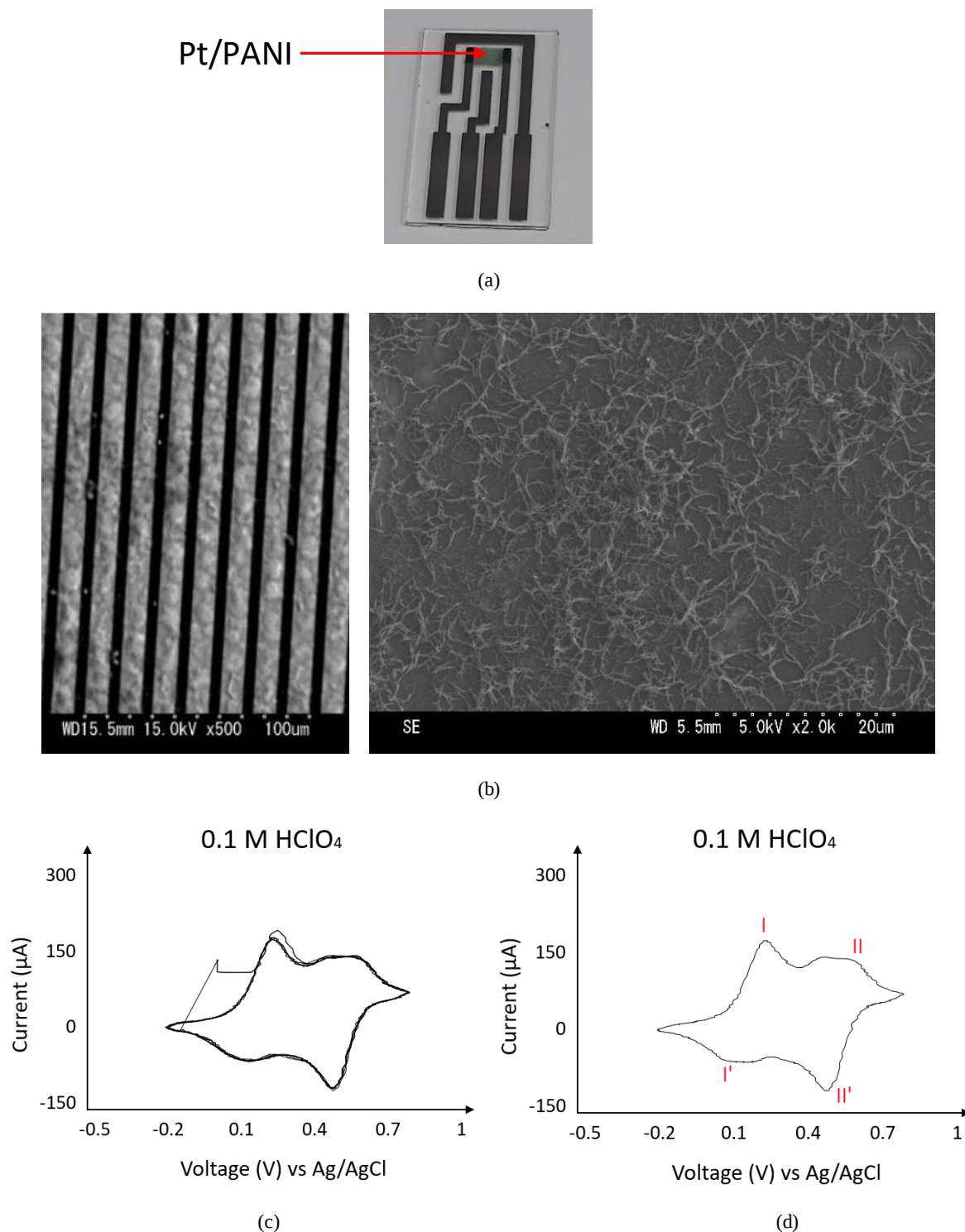
Figure 5.1: The modified working electrodes at IDA: (a) Pt/PANI working electrode; (b) the SEM image of Pt/PANI composites; (c) the curves of Pt/PANI in 0.1 M HClO 4 with 10 CVs, (d) the last CV shown from 10 CVs scanned, scan rate was 50 mV/s. Reprinted from [93]
