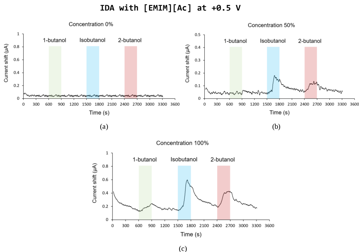
Figure 4.9: The sensor response for IDA with [EMIM][Ac] at E of +0.5 V vs. Ag/AgCl against butanol isomers at: (a) concentration of 0%; (b) concentration of 50%; (c) and concentration of 100%
