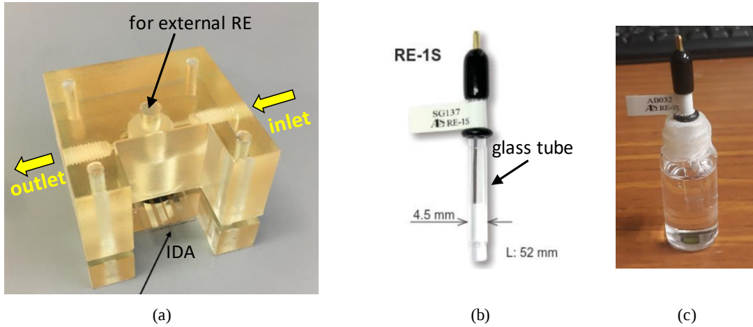
Figure 3.3: Chamber for atomic gold deposition process: (a) the acrylic chamber; (b) the external RE; (c) sealing the Ag/AgCl in 3 M NaCl solution. Reprinted from [57]
