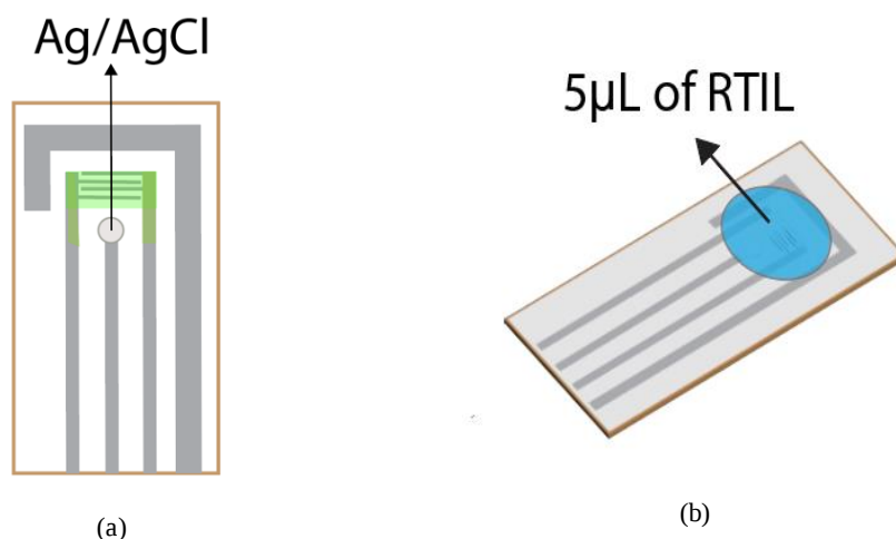
Figure 5.8: The preparation before gaseous butanol isomer measurements: (a) Ag/AgCl ink painted and dried on RE of IDA; (b) 5 \mu L of RTIL dropped on IDA surface. Reprinted from [93]
