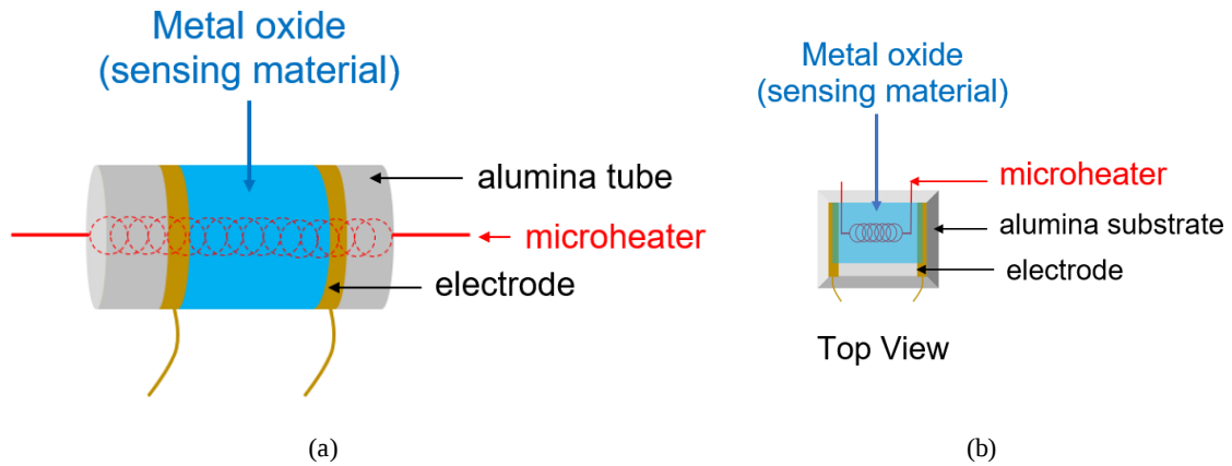
Figure 1.12: Schematic of Taguchi sensor: (a) tubular model; (b) a thin MO coated on alumina substrate
