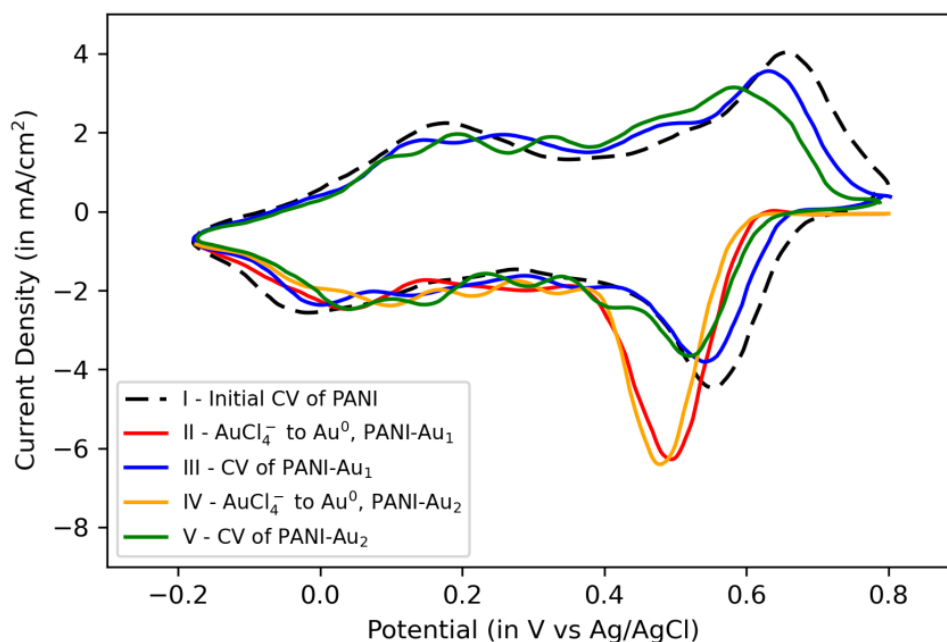
Figure 2.16: The CV of PANI in 0.1 M HClO 4 at different conditions: (I) PANI before deposition; (II) Reduction AuCl 4 - to Au in PANI; (III) CV of PANI-Au 1 ; (IV) Reduction AuCl 4 - to Au in PANI; (V) CV of PANI-Au 2 . The scan rate = 20 mV/sec. Reproduced from [57]
