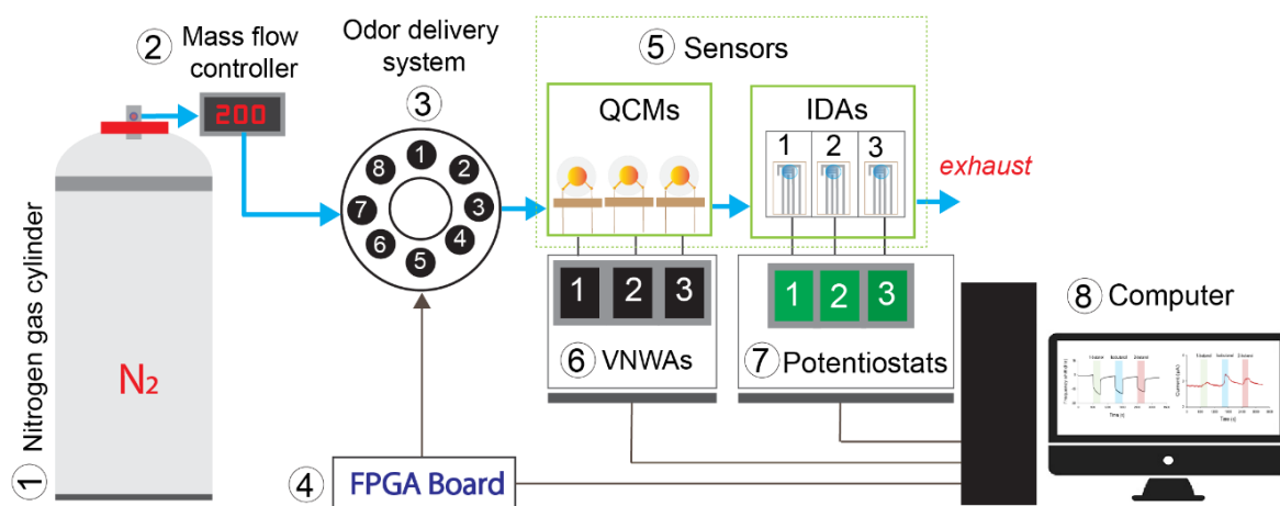
Figure 3.7: The schematic layout of gas delivery system used in this study. Reprinted from [93]
