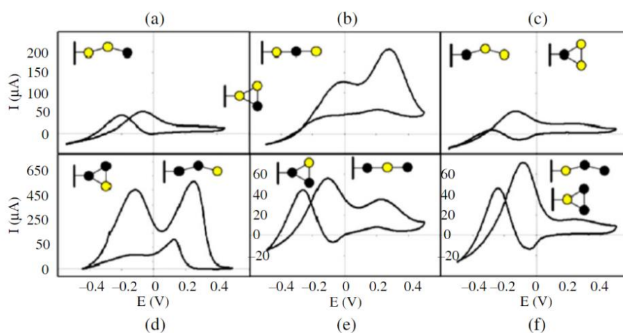
Figure 7.4: CVs for the atomic alloy, gold (Au) atom represented in yellow color, palladium (Pd) atom in black color: (a), (b), (c) are possible structures for \text{Au}_2\text{Pd}_1 , (d), (e), (f) are possible structures for \text{Pd}_2\text{Au}_1 . Reproduced from [132] with permission from Springer Nature
