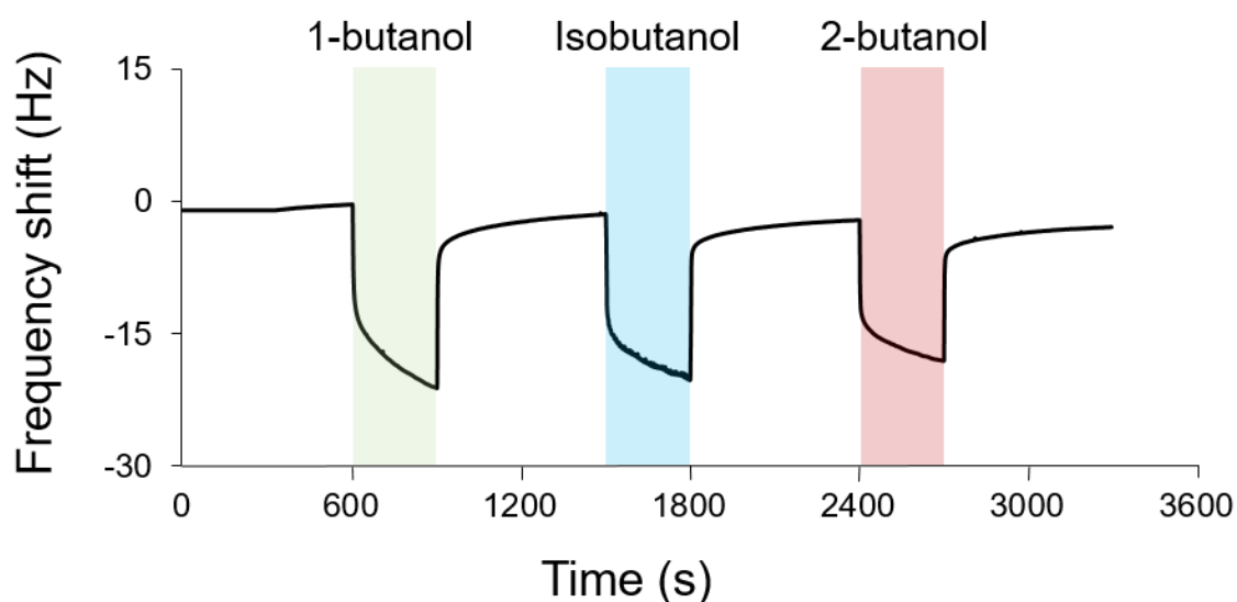
Figure 4.3: Sensor response from QCM coated with [EMIM][Ac] against 100% RC of butanol isomers. Reprinted from [98]
