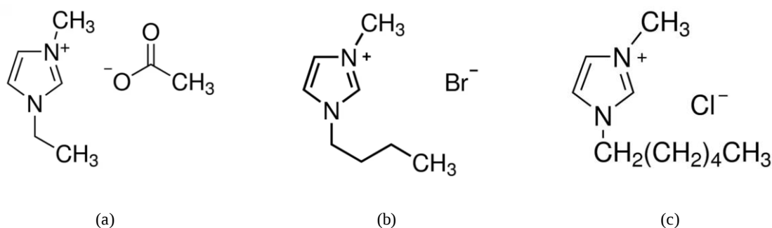
Figure 4.1: The molecular structure of RTILs used in this study: (a) [\text{EMIM}][\text{Ac}] ; (a) [\text{BMIM}][\text{Br}] ; (a) [\text{HMIM}][\text{Cl}] . Reprinted from [106–108]
