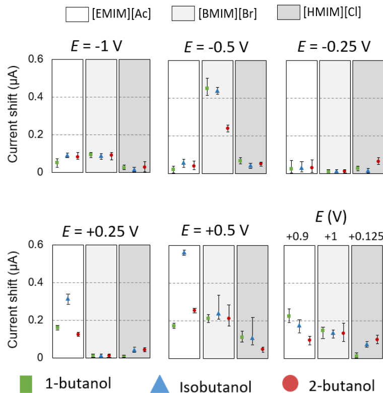
Figure 4.7: Sensor response of 100% RC butanol isomers using: (a) QCM with 3 RTILs to check the solubility of analytes during gas measurements; (b) IDAs coated with different RTILs i.e., [EMIM][Ac], [BMIM][Br], and [HMIM][Cl] at several E s vs. Ag/AgCl from 5 times measurements. Each waveform for IDAs was put in Appendix. Reprinted from [98]
