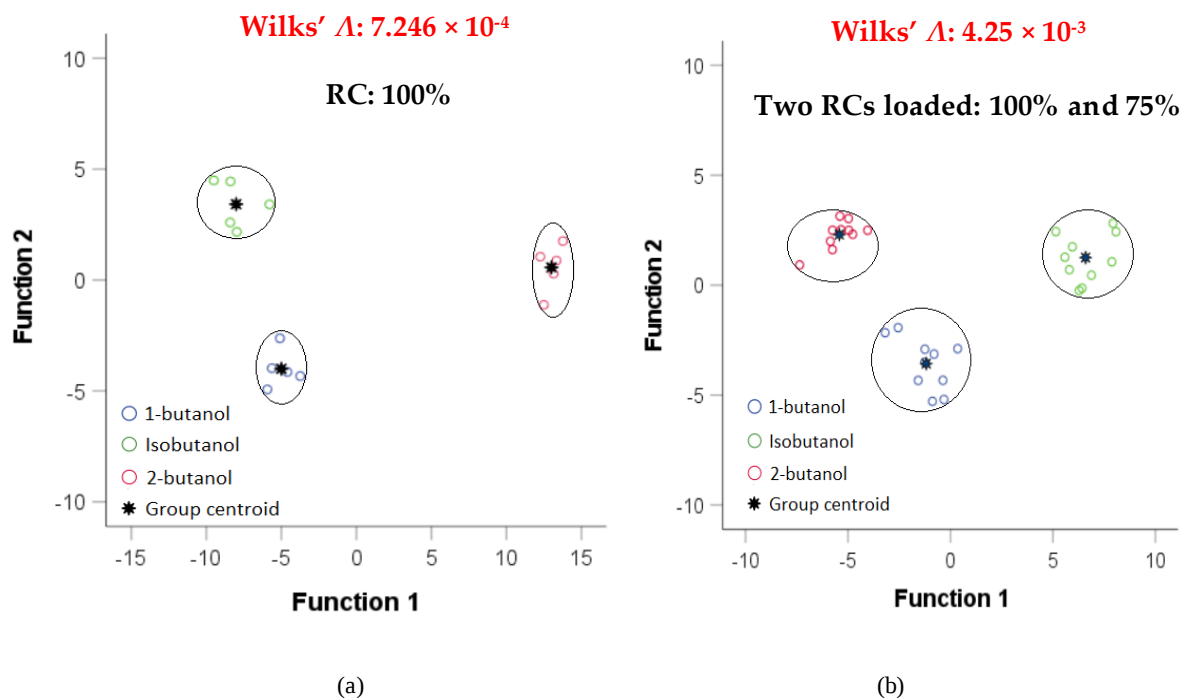
Figure 5.13: The LDA plot for selected sensing films from two sensor types, i.e., QCMs coated with [EMIM][Ac], [EMIM][Otf], [EMIM][Cl], and IDAs with [EMIM][Ac], [EMIM][Otf], [EMIM][Cl] at same E of +0.5 V vs. Ag/AgCl against butanol isomers with different concentrations: (a) RC of 100%; (b) two RCs loaded, i.e., 100% and 75%
