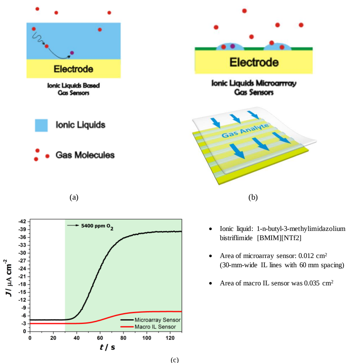
Figure 7.2: The ionic liquids applied in miniaturized AGS: (a) macro sensor; (b) microarray sensor; (c) current density-time ( J - t ) responses from microarray sensor vs. macro IL sensor. Reprinted from [131]
