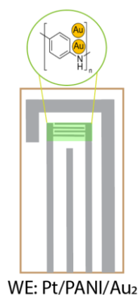
Figure 5.2: Atomic gold deposition: (a) CV curve of Pt/PANI with Au 0 , Au 1 , and Au 2 on the same IDA electrode in 0.1 M HClO 4 with scan rate of 50 mV/s; (b) Pt/PANI/Au 2 after deposition process, a thin double-sided tape was glued between IDA's substrate and acrylic chamber to maintain the IDA's position during the atomic gold deposition process. Reprinted from [93]
