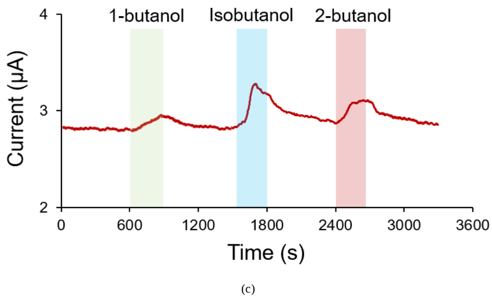
Figure 4.6: Sensor response from IDA coated with [EMIM][Ac] against 100% RC of butanol isomers at several fixed EC potential vs. Ag/AgCl: (a) -1 V; (b) -0.25 V; (c) +0.5 V. Reprinted from [98]
