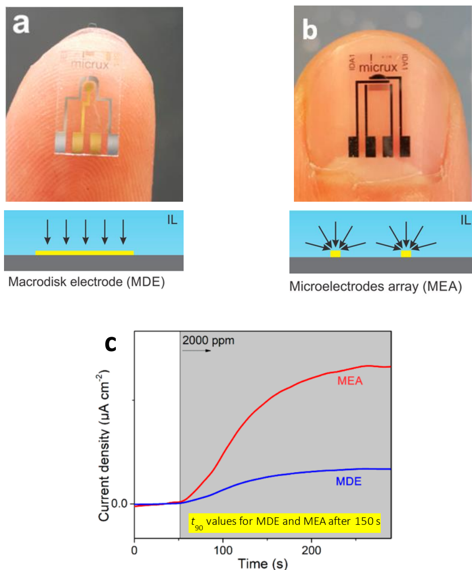
Figure 1.18: Miniaturized AGS system with RTIL: (a) MDE configuration; (b) MEA configuration; (c) the response time of MDE (blue) and MEA (red) for \text{O}_2 at 2000 ppm concentration. Reprinted with permission from [41]. Copyright 2017 American Chemical Society
