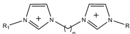
1,3-bis[3-methylimidazolium-1-yl]alkane
