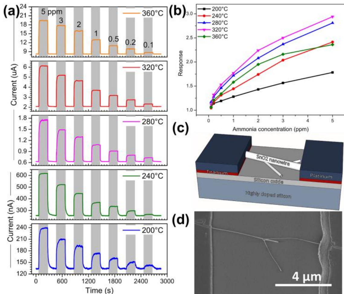
Figure 1.24: A single \text{SnO}_2 nanowire applied for ammonia gas measurement: (a) the sensor responses for different concentrations of gaseous ammonia (5 ppm, 3 ppm, 2 ppm, 1 ppm, 0.5 ppm, 0.2 ppm, 0.1 ppm) at different temperatures (200 °C, 240 °C, 280 °C, 320 °C, 360 °C); (b) sensor response as a function of various concentration of ammonia with different temperatures; (c) 3D-model of sensor with a single \text{SnO}_2 nanowire; (d) the SEM image. Reproduced from [49]
