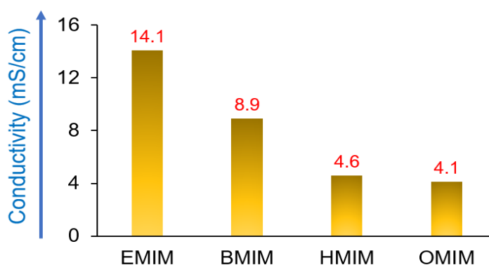
Figure 2.6: The variation of conductivity from several alkyl chain length using imidazolium cation-based RTILs. Reproduced from [73] with permission from the Royal Society of Chemistry
