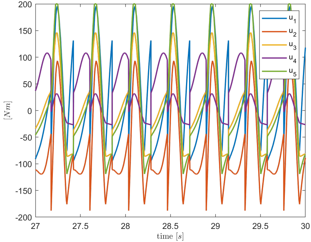
Figure 2.10: Motor torques
