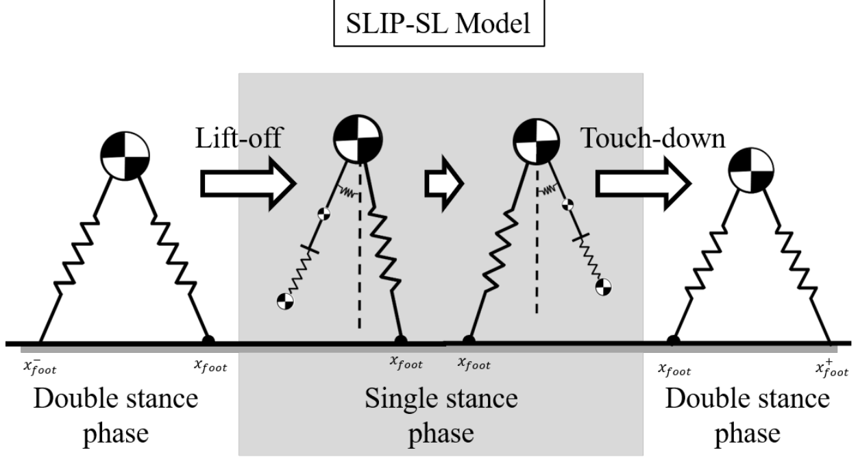
Figure 2.4: SLIP-SL Model
