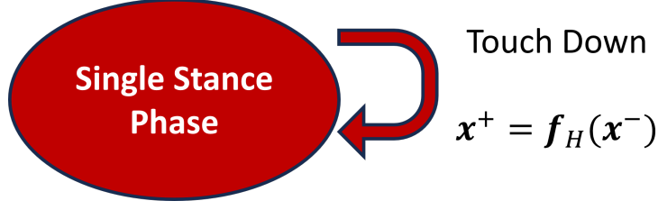
Figure 5.4: State transition
