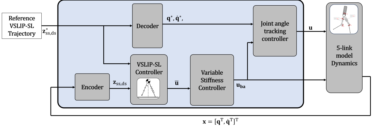
Figure 7.4: Controller diagram for the variable stiffness BA model
