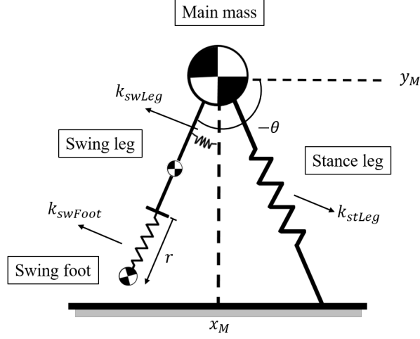
Figure 2.1: SLIP-SL Model in the single stance phase
