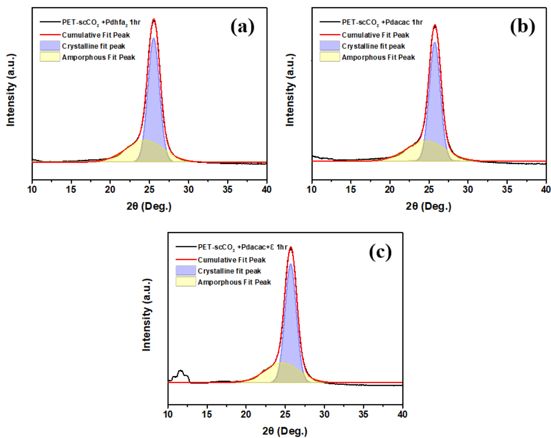
Figure 7-4. XRD patterns of the (a) PET film treated by sc-CO 2 with Pd(hfa) 2 , (b) Pd(acac) 2 , and (c) Pd(acac) 2 + \epsilon -caprolactam for 1 hr.
