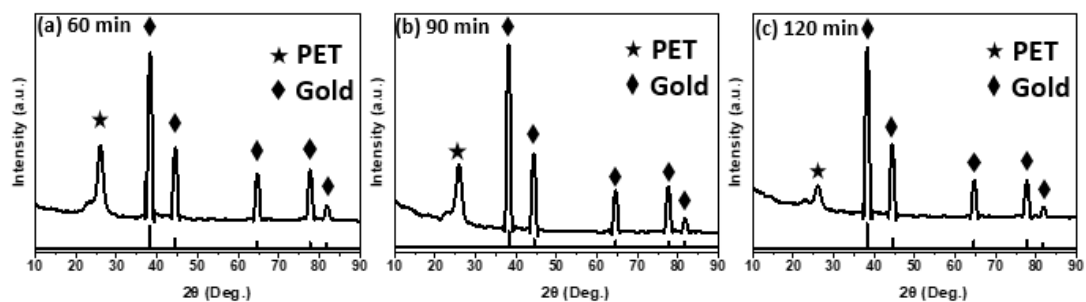
Figure 2-8. XRD of Au/Ni-P/PET composites with (a) 60.0, (b) 90.0 and (c) 120.0 min of the gold deposition time. (FCC Au: JCPDS no. 04-0784)
