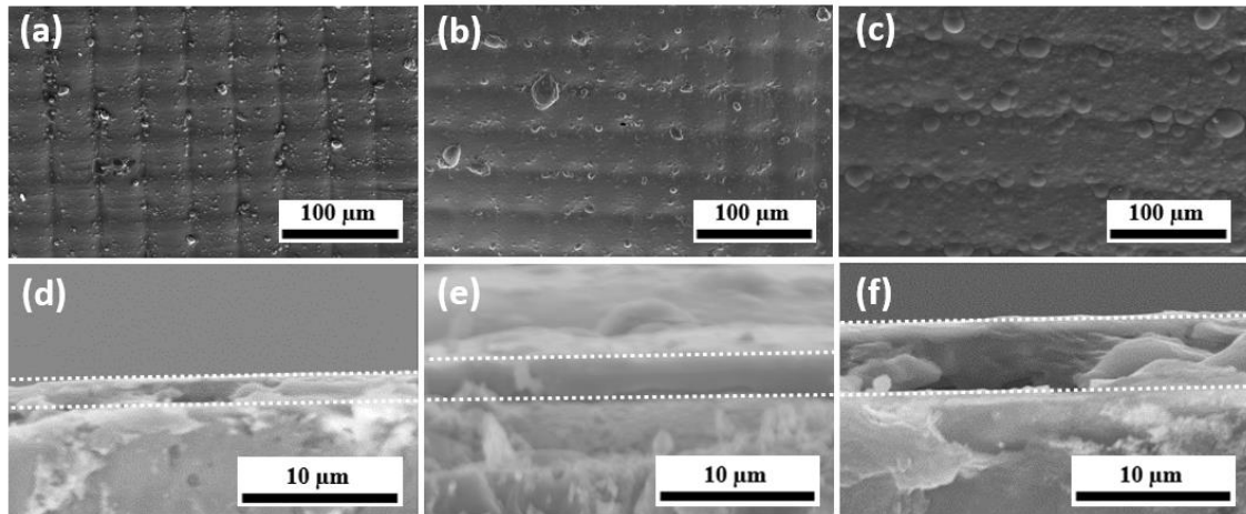
Figure 4-3. Surface morphology of Ni-P metallized 3D-printed square-pad structures treated by the sc-CO 2 catalyzation follow by (a) 3, (b) 10, and (c) 30 min of the metal deposition time, and cross-sectional view of the samples with (d) 3, (e) 10, and (f) 30 min of the metal deposition time and the deposition temperature at 90 °C.
