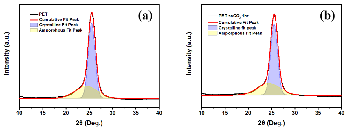
Figure 7-2. XRD patterns of the (a) PET film and the PET film treated by \text{sc-CO}_2 for (b) 1hr.
