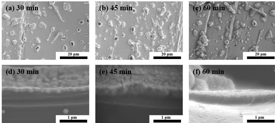
Figure 3-3. Surface morphology of Pt metallized PET treated by the sc-CO 2 catalyzation follow by (a) 30 min, (b) 45 min, and (c) 60 min of the Pt deposition time, and cross-sectional view of the specimen with (d) 30 min, (e) 45 min, and (f) 60 min of the Pt deposition time.
