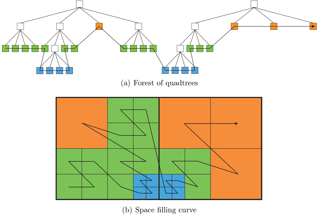
Figure 5.1: Tree-Based Block-Structured AMR.
