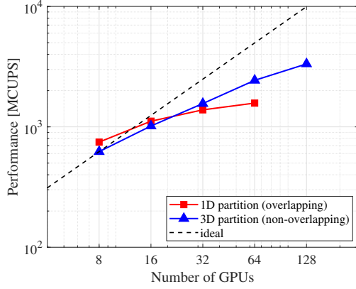
Figure 4.6: Comparison between 1D domain partition (overlapping) and 3D domain partition (non-overlapping) for the strong scaling of Con-CAC-LS on a 512 \times 512 grid.
