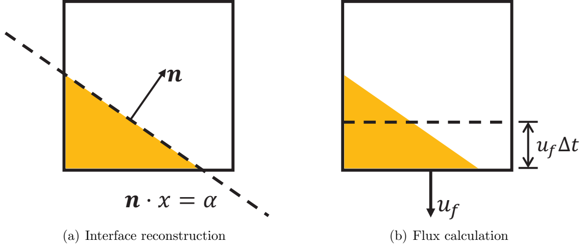
Figure 4.1: PLIC method.
