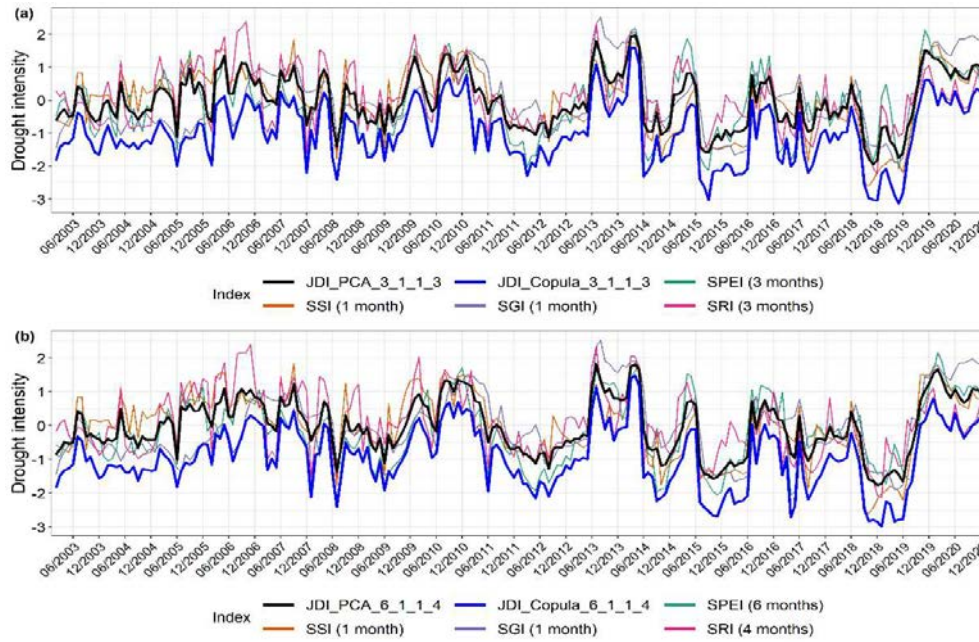
Figure 3.11: Time series of JDI_PCA and JDI_Copula during 2003 to 2020 for scales (a) 3_1_1_3 and (b) 6_1_1_4, where the scales are in the order of SPEI, SSI, SGI, and SRI, along with time series of the integrated indices SPEI, SSI, SGI, and SRI with their respective scales.
