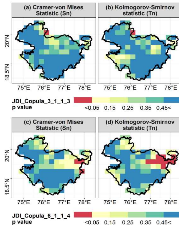
Figure 3.9: Significance value ( p value) for Cramer-von Mises statistic (Sn) and Kolmogorov-Smirnov statistic (Tn) for gaussian copula in Kharif season (a & b; JDI_Copula_3_1_1_3) and Rabi season (c & d; JDI_Copula_6_1_1_4).
