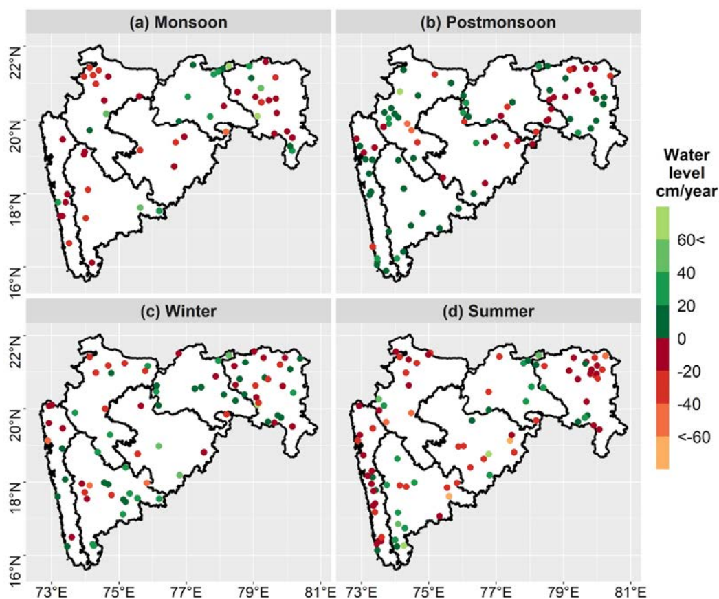
Figure 2.14: Significant trend in well levels by MK trend analysis ( p<0.05 ) in each season; (a) monsoon, (b) postmonsoon, (c) winter, and (d) summer over the state. The in-situ groundwater table data shows significant decreasing or increasing trends in all parts of the state in each season, signifying the localized and seasonal influence of groundwater abstraction.
