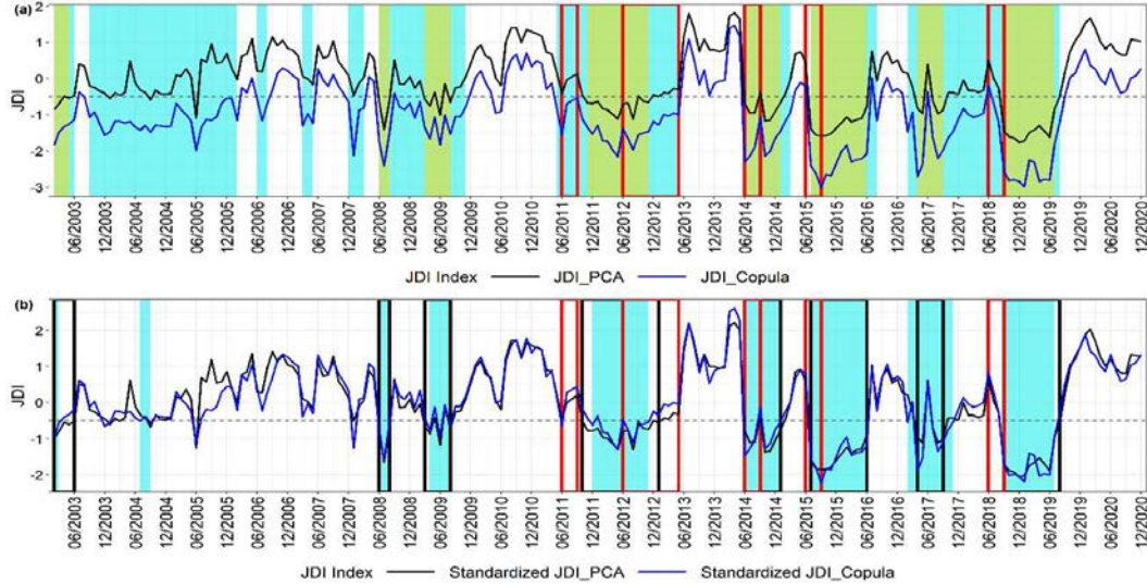
Figure 3.22: (a) Continuous time series of JDI_PCA and JDI_Copula from 2003 to 2020 with scale 3_1_1_3 for June–September and scale 6_1_1_4 from October to May. Green and blue shaded regions represent drought periods for JDI_PCA and JDI_Copula, respectively, where green areas overlap blue areas each time. (b) Continuous time series of standardized JDI_PCA and standardized JDI_Copula. Black rectangles represent drought events in standardized JDI_PCA while blue shaded regions represent drought events in standardized JDI_Copula. In both subfigures, JDI intensity below -0.5 is considered as drought event and red rectangles show the declared drought events mentioned in Table 3.7.
