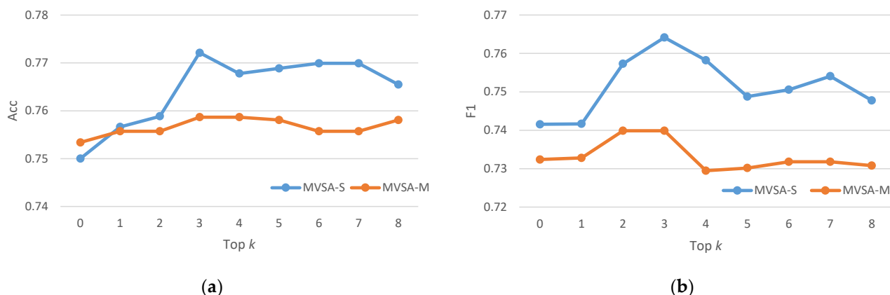
Figure 4. The experimental results for different values of hyperparameter k . (a) The accuracy of GLFN with different top k . (b) The F1-score of GLFN with different top k .
