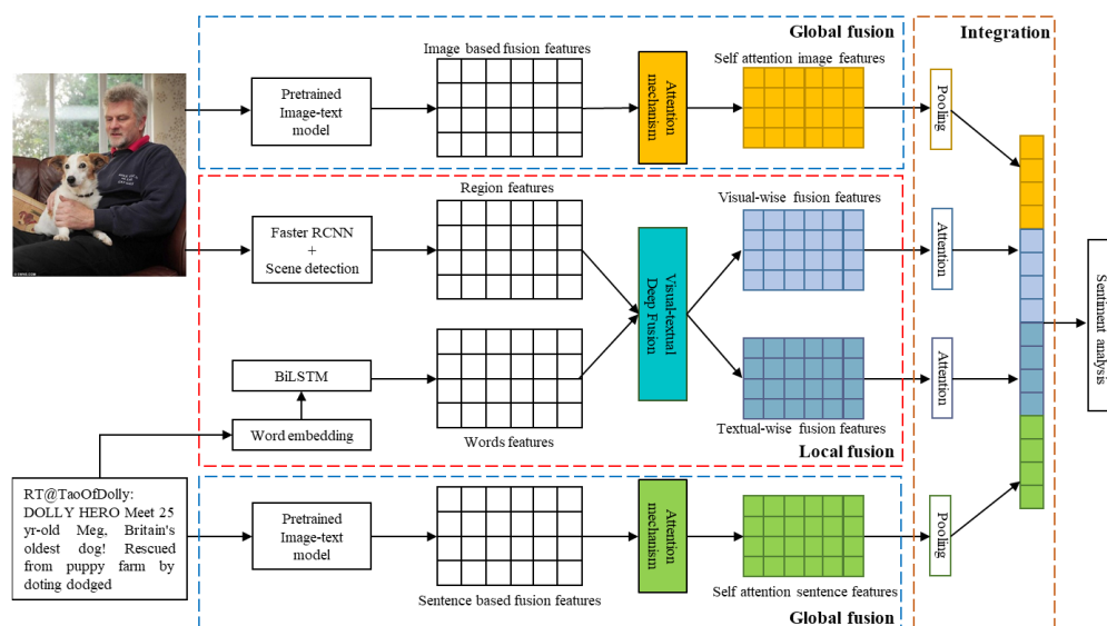
Figure 2. The overall framework of proposed model.
