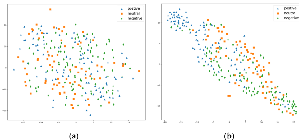
Figure 5. Visualization results of visual features projected to two-dimensional space. (a) Visualization of the initial visual features. (b) Visualization of the attention-based features.
