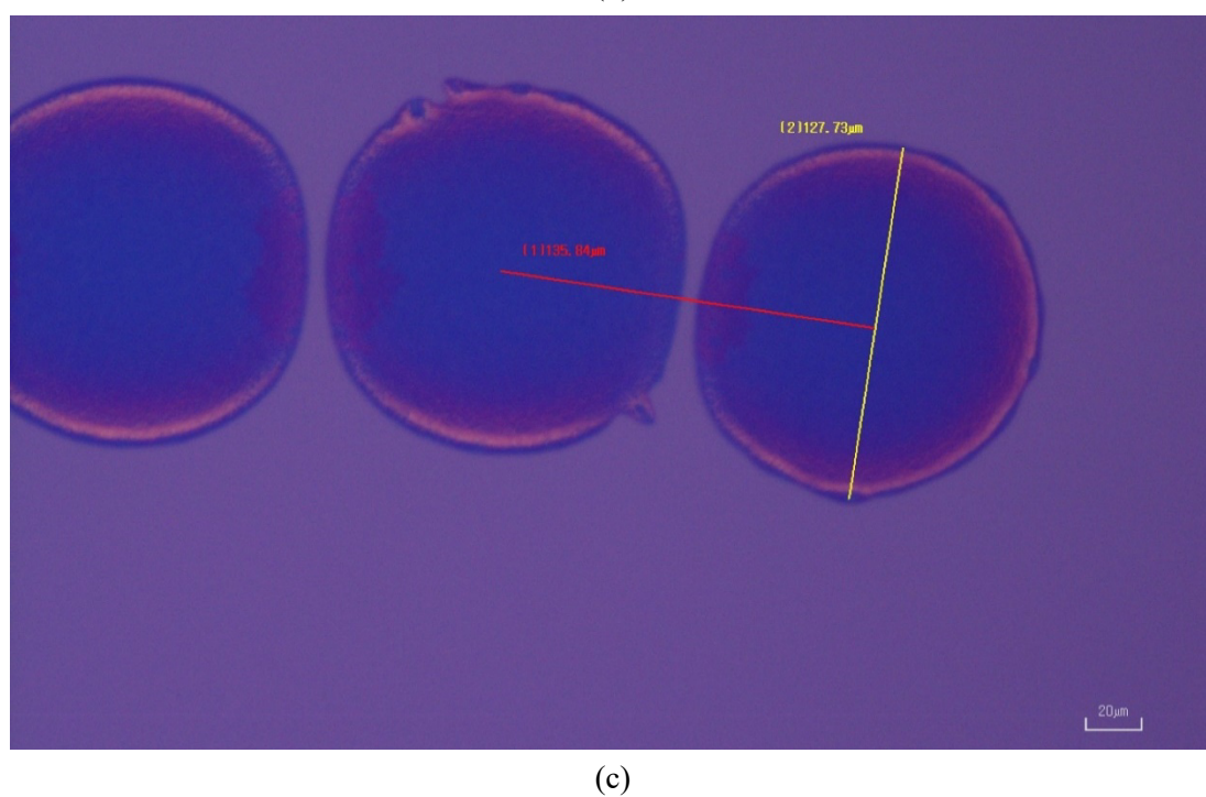
Figure. 5.4 Images of inkjet-printed silver dot (a, b) before and (c) after sintering. Drop spacing is 135 \mu\text{m} and the number of dot is 13.
