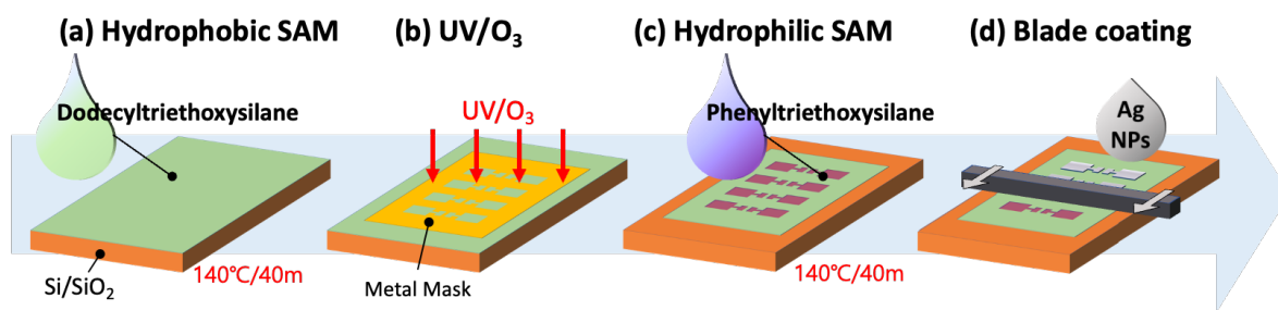
Figure. 5.6 Conceptual illustration of the patterning process using differential surface energy with the hydrophobic and hydrophilic SAMs materials dodecyltriethoxysilane (DTS) and phenyltriethoxysilane (PTS), respectively. (a) DTS was drop-casted. (b) DTS was oxidized by exposure to UV light in an ozone atmosphere. (c) PTS was drop-casted. (d) Silver nanoparticles (AgNPs) ink was blade coated.
