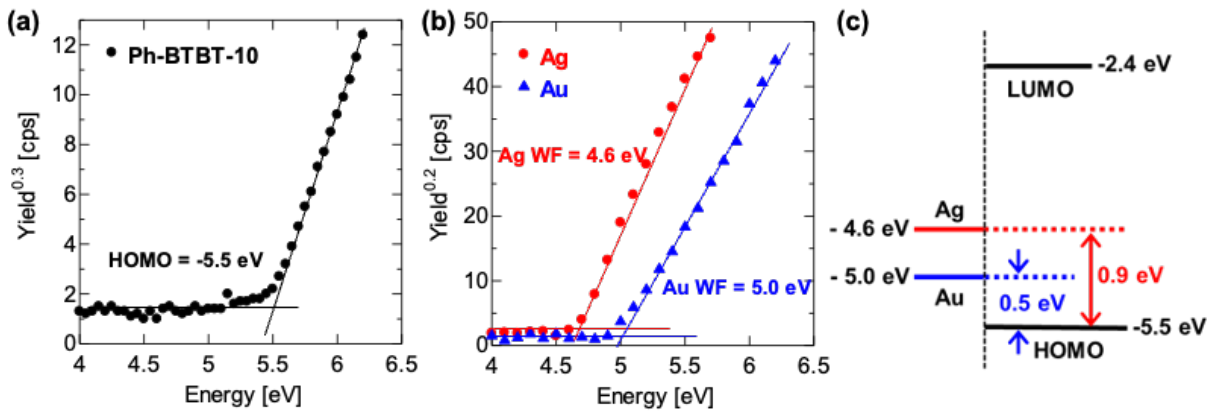
Figure 3.6 (a) The highest occupied molecular orbital (HOMO) of Ph-BTBT-10 (b) Work functions (WF) of silver and gold electrodes, respectively. (c) Energy diagram of the HOMO level of Ph-BTBT-10 and the work functions of silver and gold.
