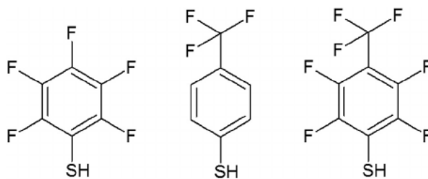
Figure 4.10 Chemical structures of SAM materials. (a) PFBT, (b) TFBT, and (c) TTFP.
