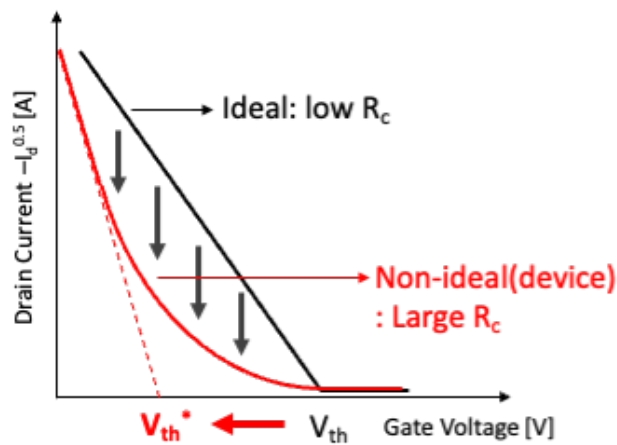
Figure 3.4 Conceptual illustration for transistor characteristics of OFETs with ideal and non-ideal
