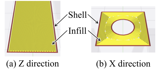
Fig. 4. Infill pattern
