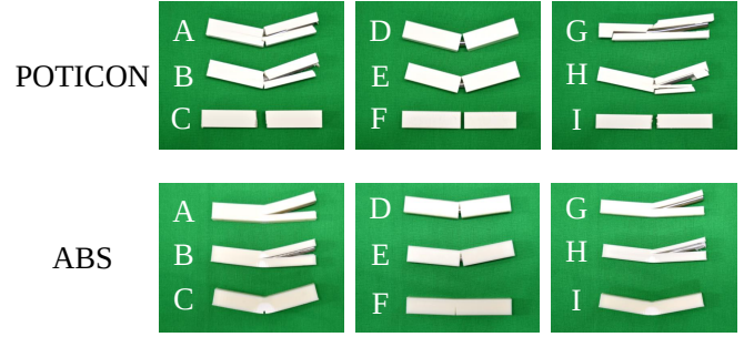
Fig. 8. Fracture specimens
