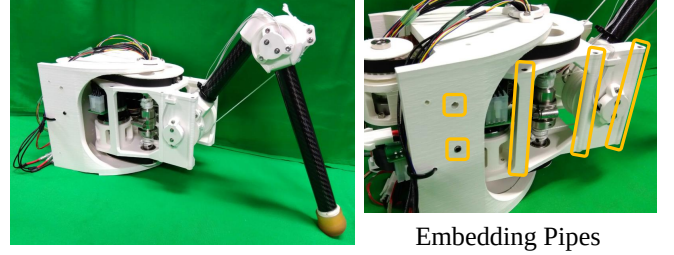
Fig. 9. Application example
