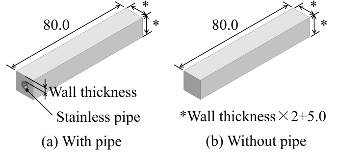
Fig. 1. Specimen
