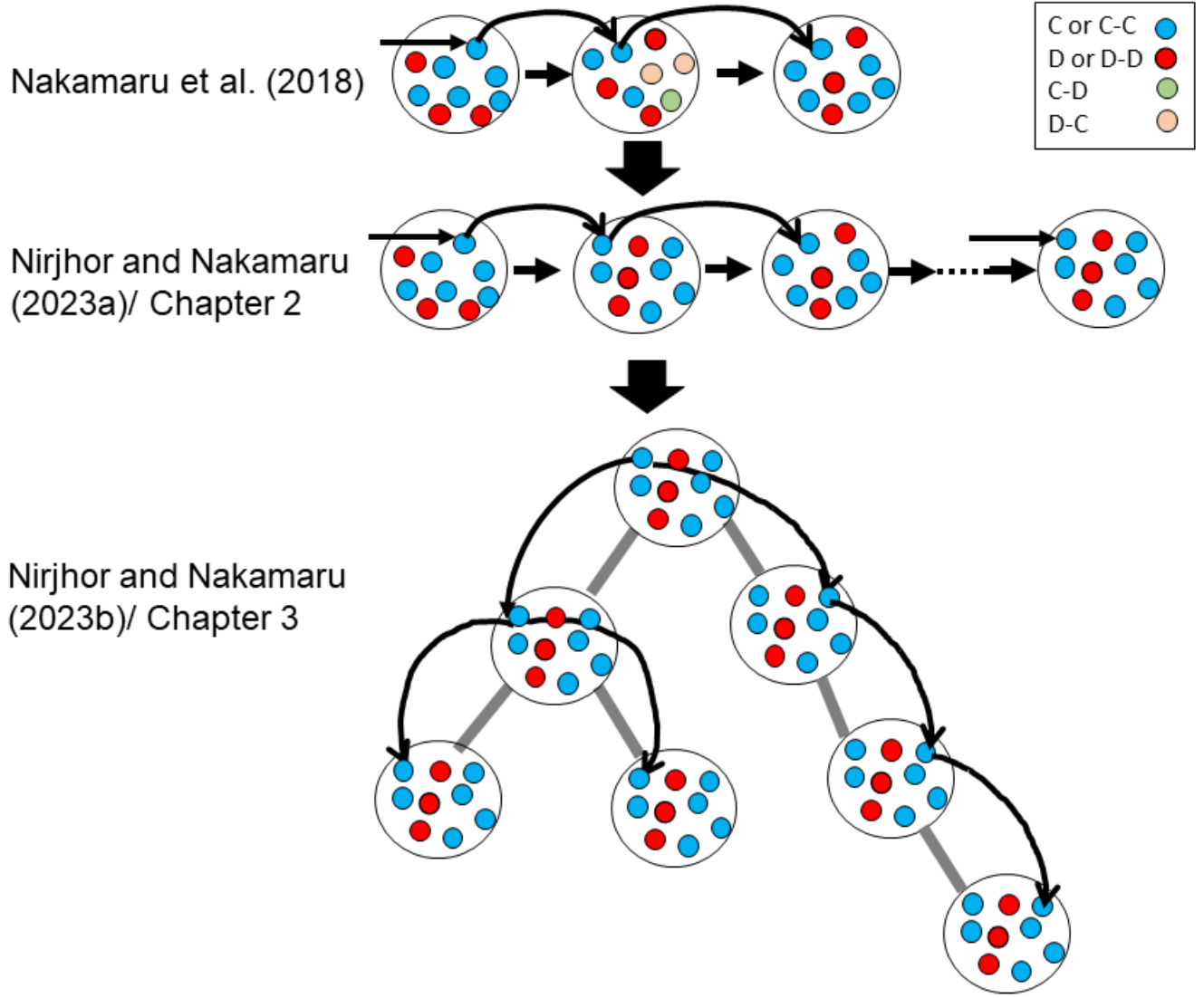
Figure 1.1: Relation of this thesis with Nakamaru et al.(2018). C is for a cooperators, D is for a defectors. In Nakamaru et al. (2018) there was only three roles, however in the 2nd group there were 4 types of strategy. In Nirjhor and Nakamaru (2023a) which corresponds to the chapter 2 in this thesis there are finite number of roles in the linear division of labour. In Nirjhor and Nakamaru (2023b) which corresponds to the chapter 3 in this thesis it is a division of labour on a finite unidirectional tree graph.
