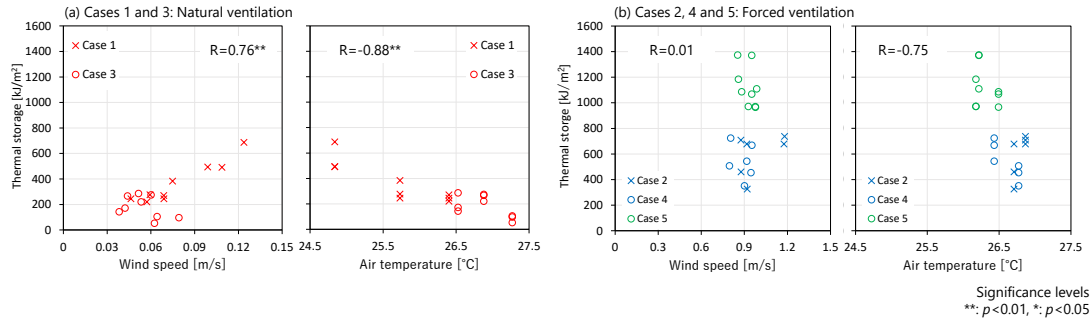
Fig. 4.14. Correlation between the thermal storage of PCM and wind speed/ mean outdoor temperature during the nighttime in case of (a) natural ventilation and (b) forced ventilation
