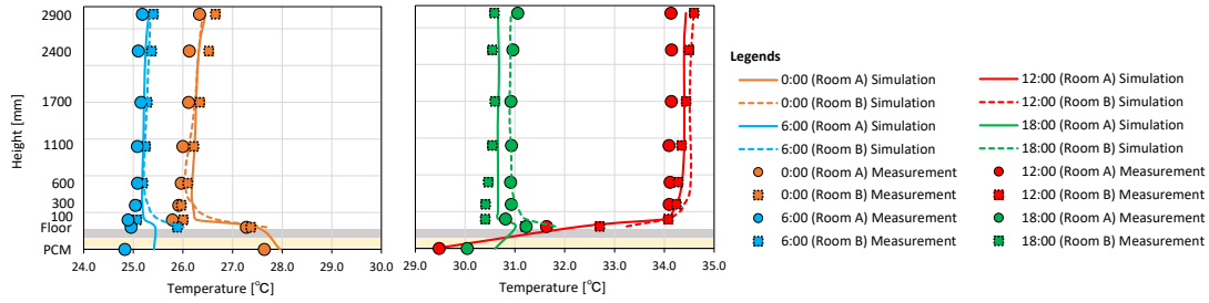
Fig. 5.6. Comparison of air temperatures between the measurement and simulation at 0:00, 6:00, 12:00, and 18:00, day 1 in Rooms A and B.
