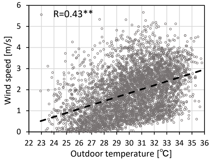
Fig. 7.13. Relationship between diurnal outdoor temperature and wind speed in the experimental site (2020).
