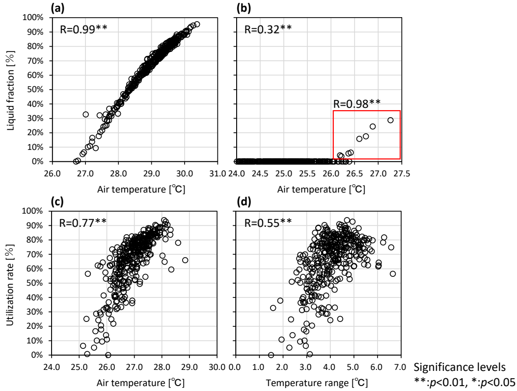
Fig. 6.15. Correlation between (a) \beta_{max} and daily maximum air temperature in the underfloor space, (b) \beta_{min} and daily minimum air temperature in the underfloor space, (c) utilization rate and daily mean temperature in the underfloor space, and (d) utilization rate and air temperature range in the underfloor space in Case 4.
