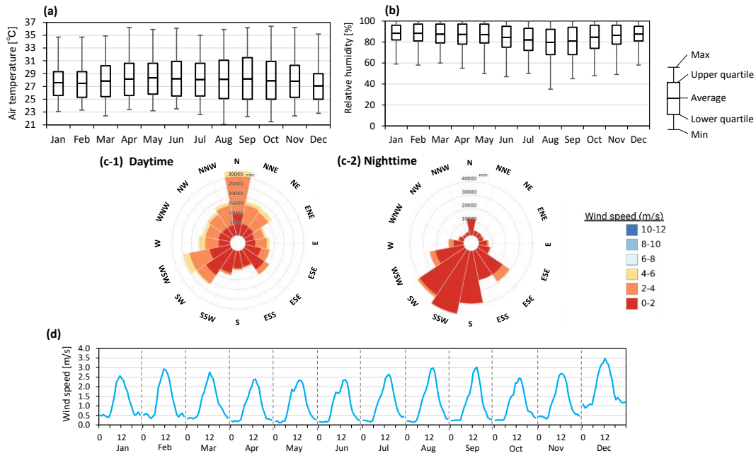
Fig. 7.4. (a) Outdoor air temperature range, (b) outdoor relative humidity range, (c) wind rose in 2020, and (d) monthly averaged daily patterns of the outdoor wind speed.
