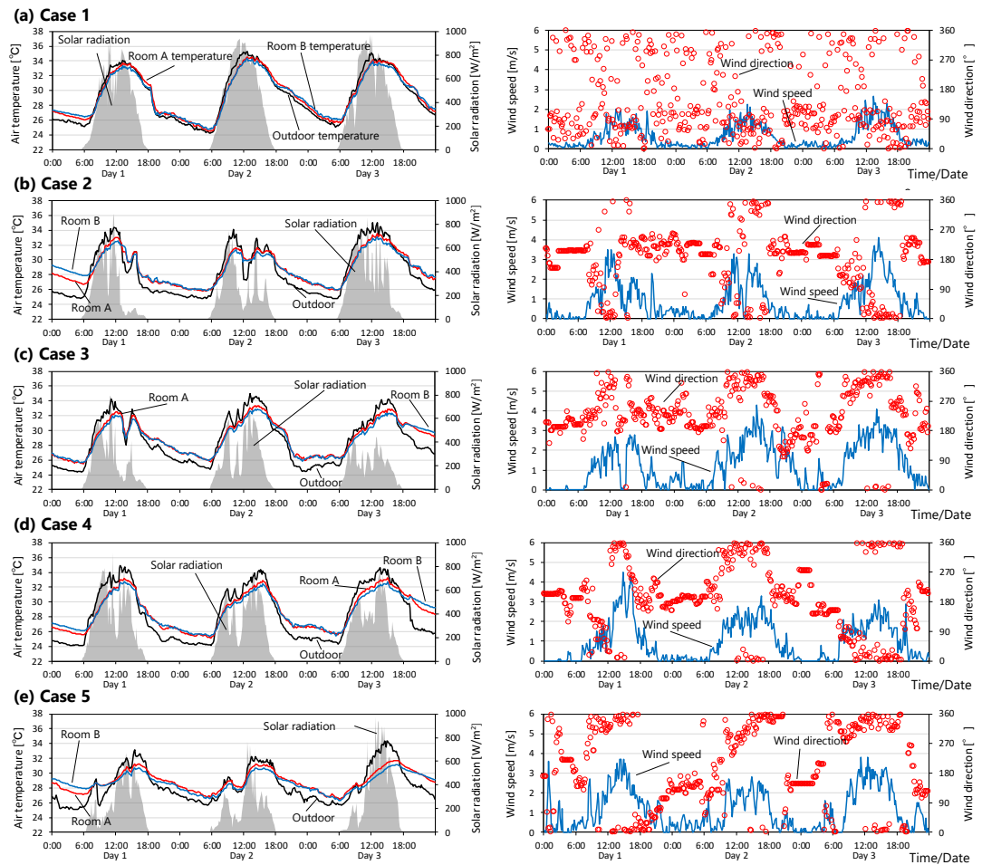
Fig. 3.4. Temporal variation of the measured air temperature in the experimental building and the corresponding outdoor conditions in Case (a) Case 1; (b) Case 2; (c) Case 3; (d) Case 4; (5) Case 5.
