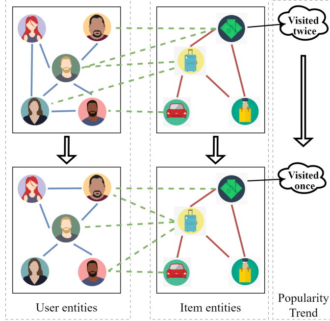
Figure 4.1: An example of a social media network consists of users and items. Solid lines denote the interactions between users and items, and dash lines denote the interactions between user-item pairs. Interactions and entity attributes evolve as time goes by. The popularity trend of an item is represented by the visit frequency, which indicates the number of accesses from users (the degree of dashed lines).
