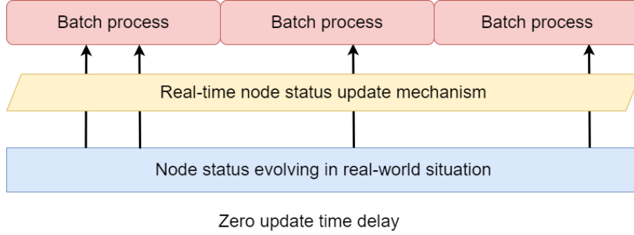
Figure 5.10: The zero update time delay in TDGNN. TDGNN has a real-time node status update mechanism that can update node information during batch process.
