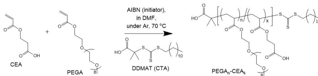
Scheme 2.3. Synthesis of PEGAn-CEAk using RAFT polymerization.
