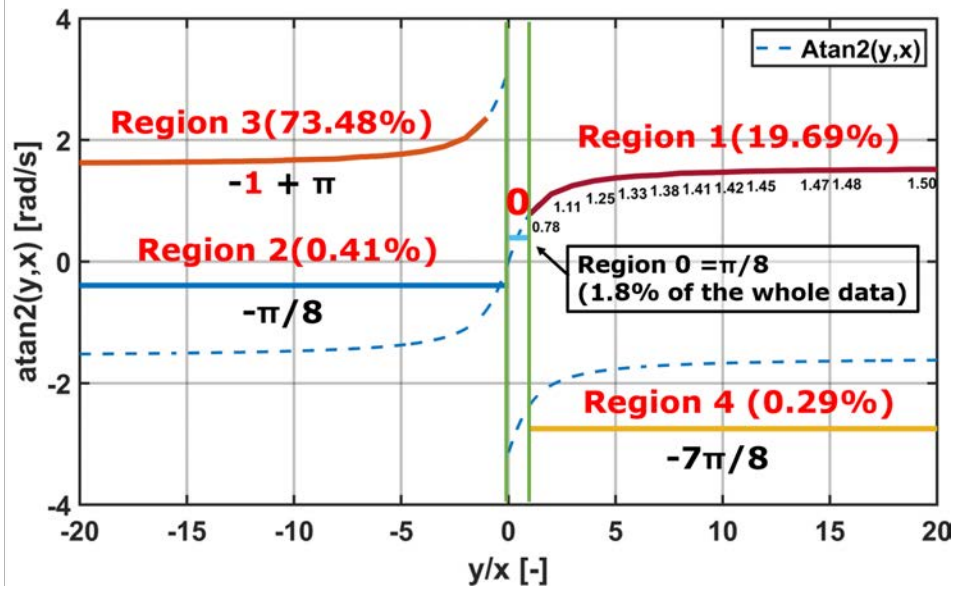
Figure 3.1: 2 argument arctangent approximation using binary search look up table and assignment of constants to regions with small portion of the overall dataset.
