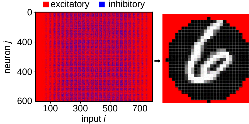
Figure 8.2: Color coded weight matrix of the synapses between input and hidden layer (left). Resulting mask on example image determined from inputs with >90\% excitatory weights assigned across the hidden layer (right).
