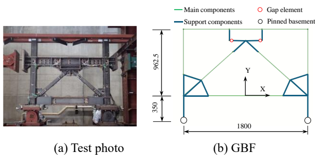
Figure 1 Test specimen and simplified model of GBF
