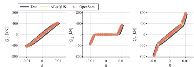
Figure 2 Q-R relationship of GBF
