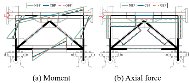
Figure 6 Moment and axial force distribution comparison
